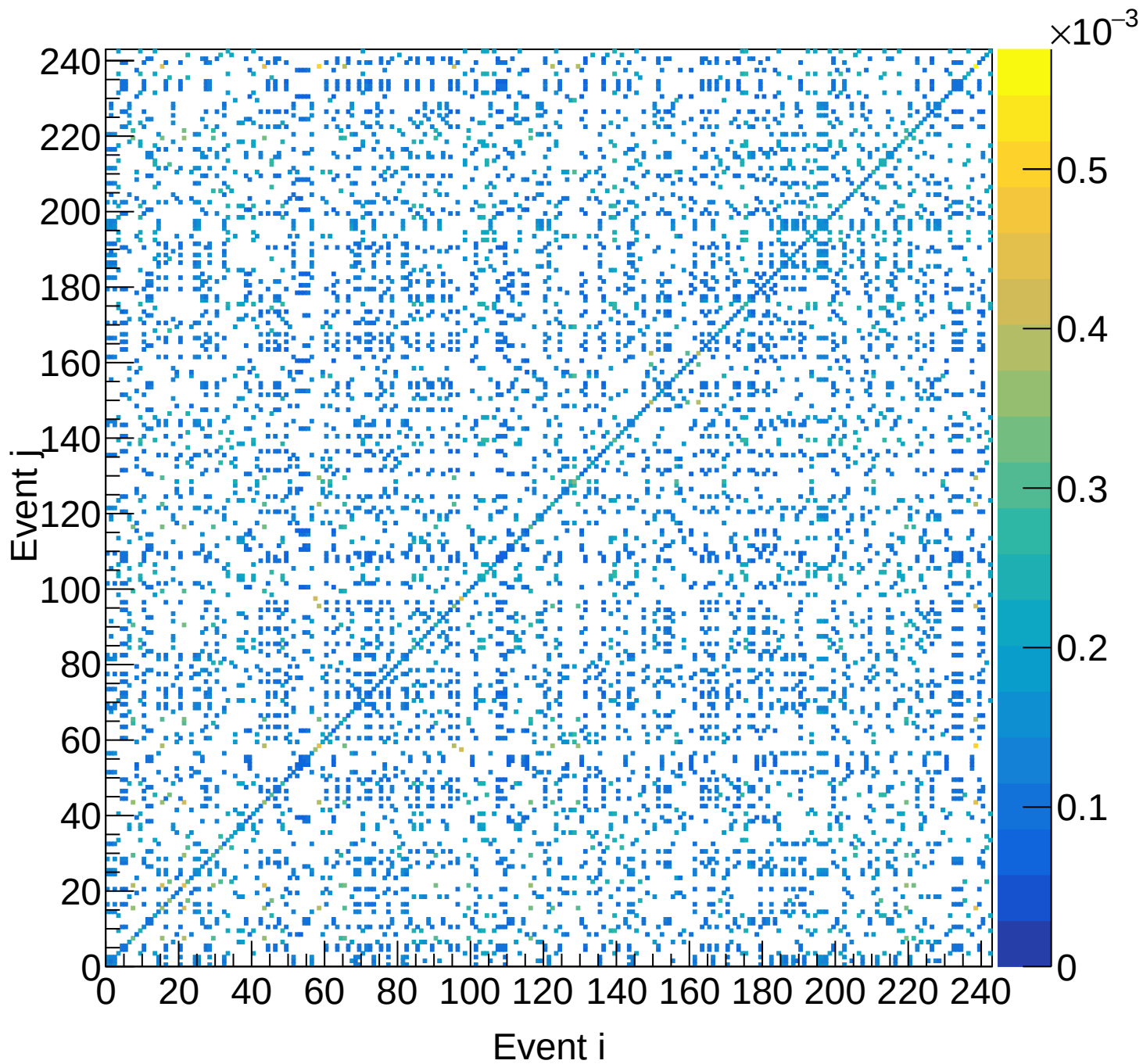
LH2 (total) Covariance | M: [5.1, 5.4) xF: [0.25, 0.30)
