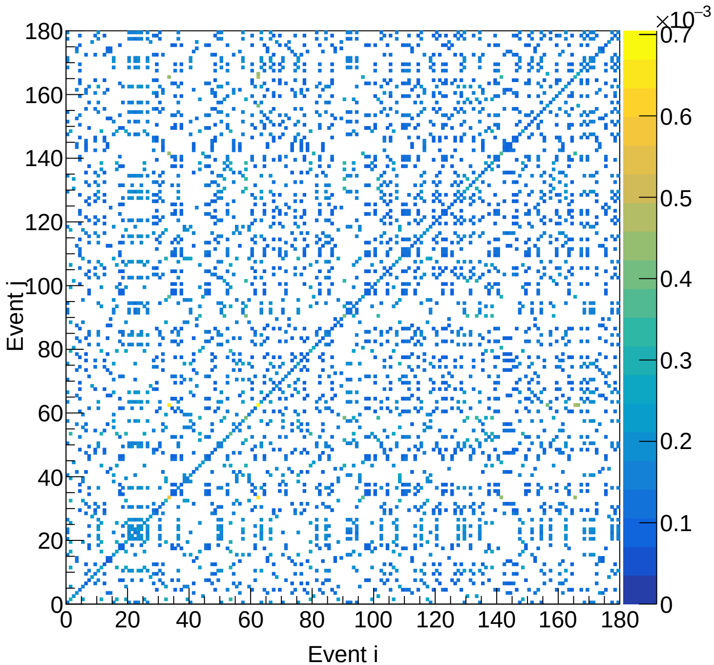
LH2 (total) Covariance | M: [5.4, 5.7) xF: [0.25, 0.30)
