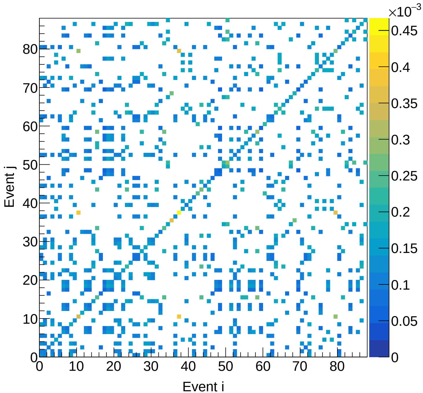
LH2 (total) Covariance | M: [5.7, 6.0) xF: [0.25, 0.30)
