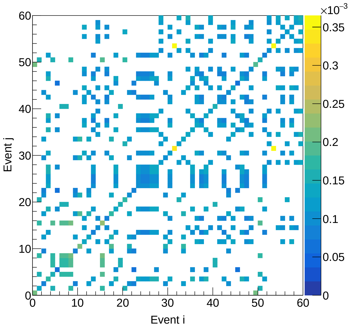
LH2 (total) Covariance | M: [6.0, 6.3) xF: [0.25, 0.30)
