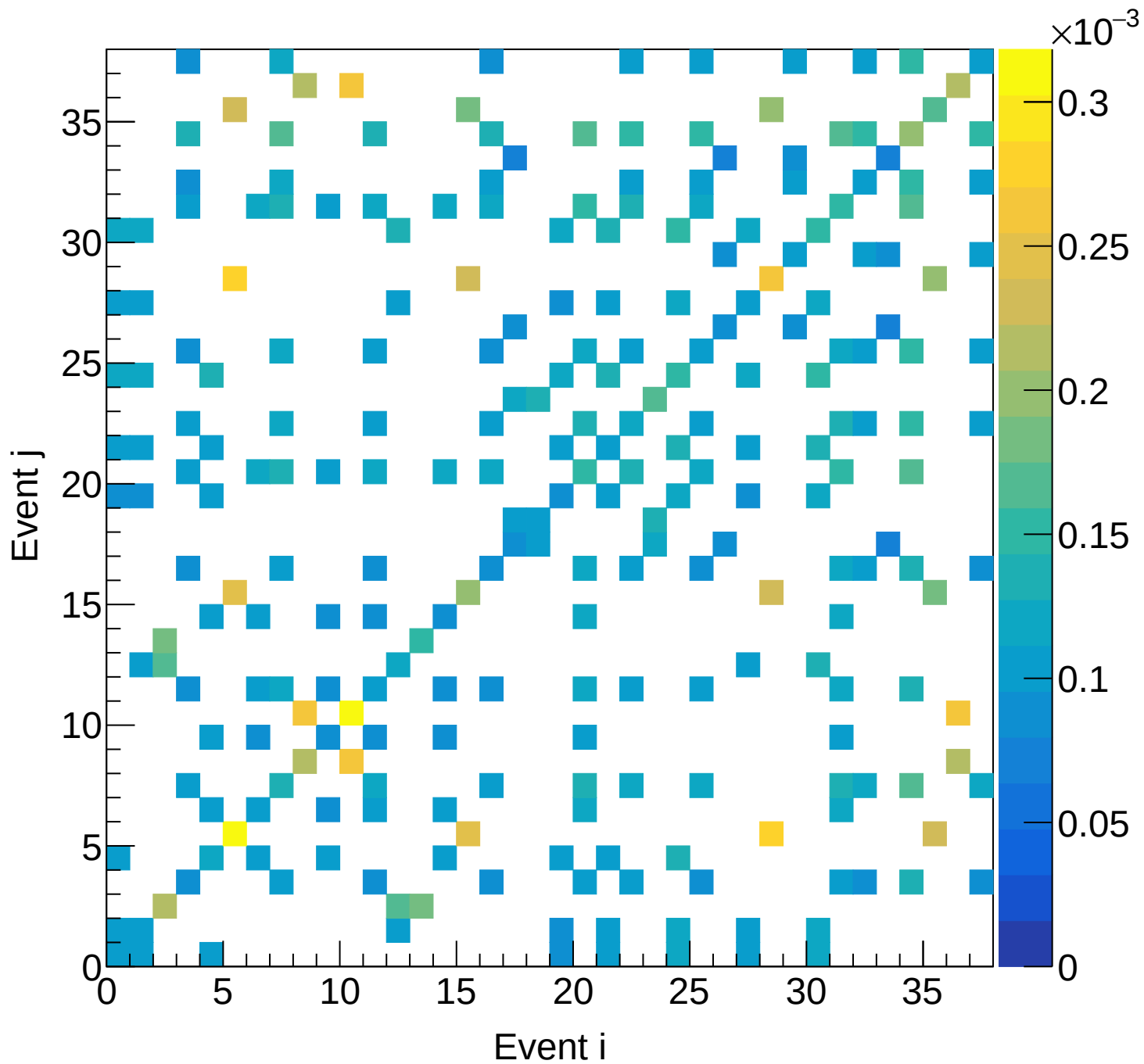
LH2 (total) Covariance | M: [6.3, 6.6] xF: [0.25, 0.30]
