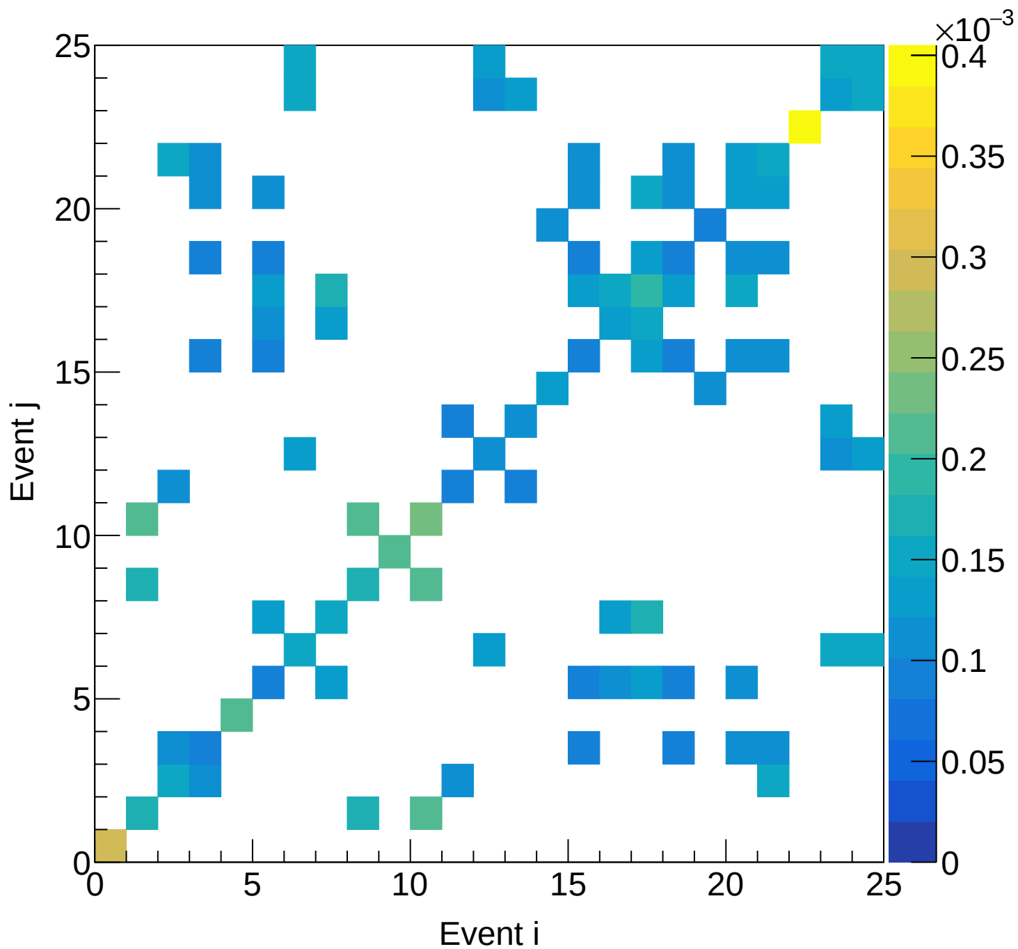
LH2 (total) Covariance | M: [6.6, 6.9) xF: [0.25, 0.30)
