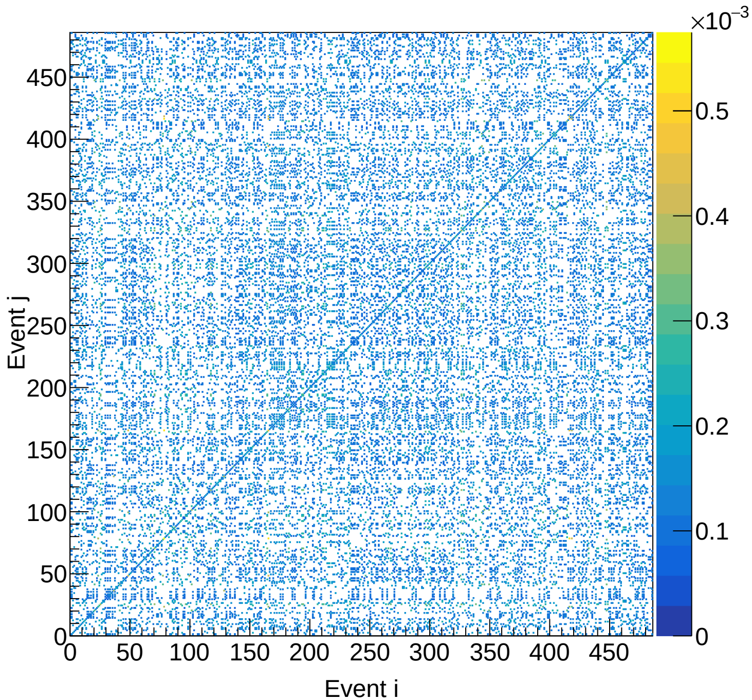
LH2 (total) Covariance | M: [3.9, 4.2) xF: [0.30, 0.35)
