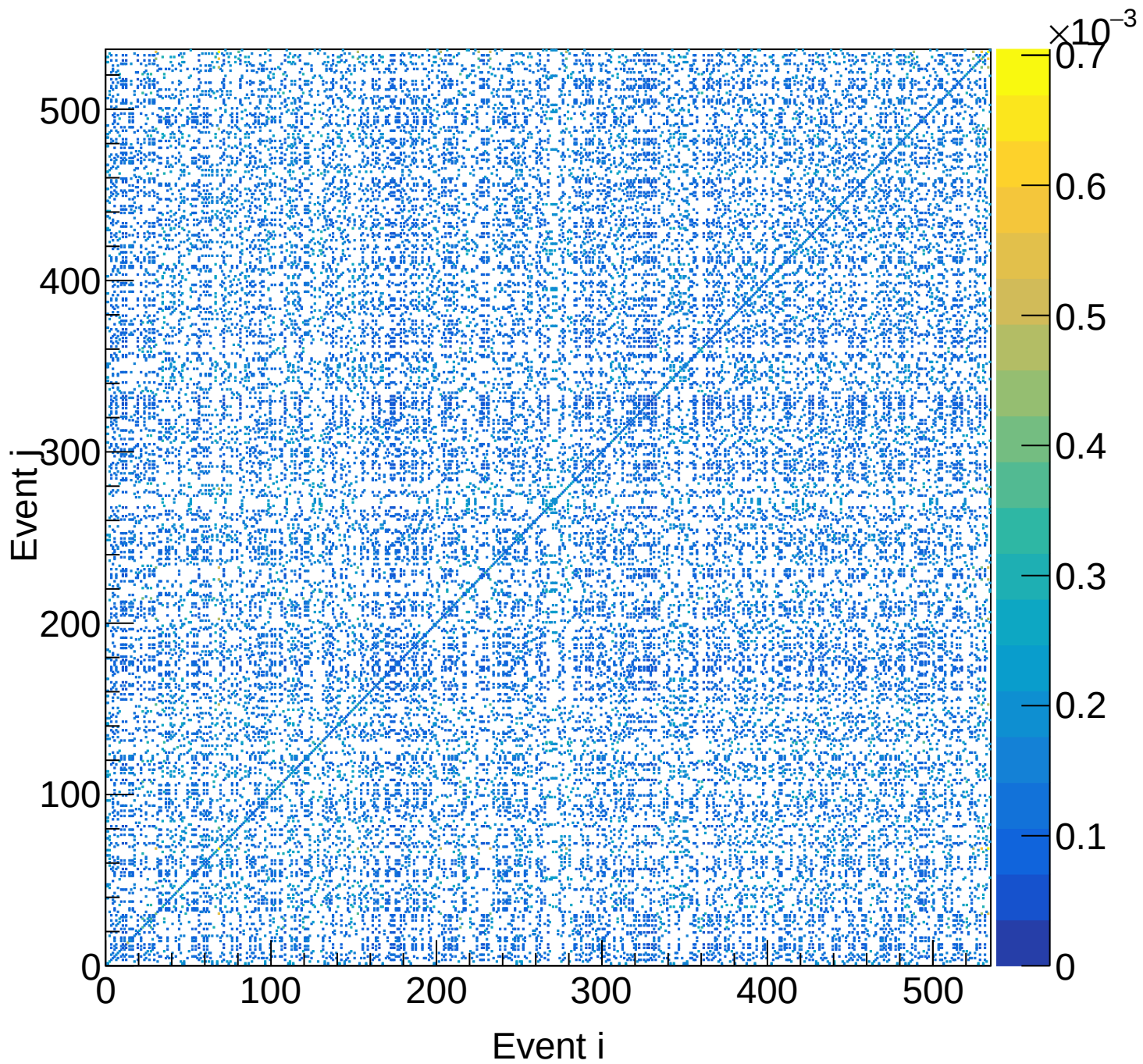
LH2 (total) Covariance | M: [4.2, 4.5) xF: [0.30, 0.35)
