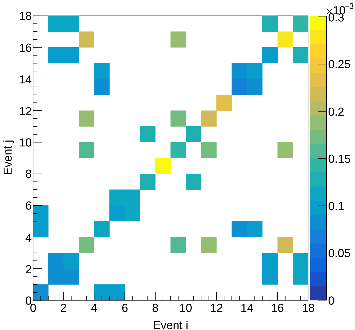
LH2 (total) Covariance | M: [6.9, 7.5) xF: [0.30, 0.35)
