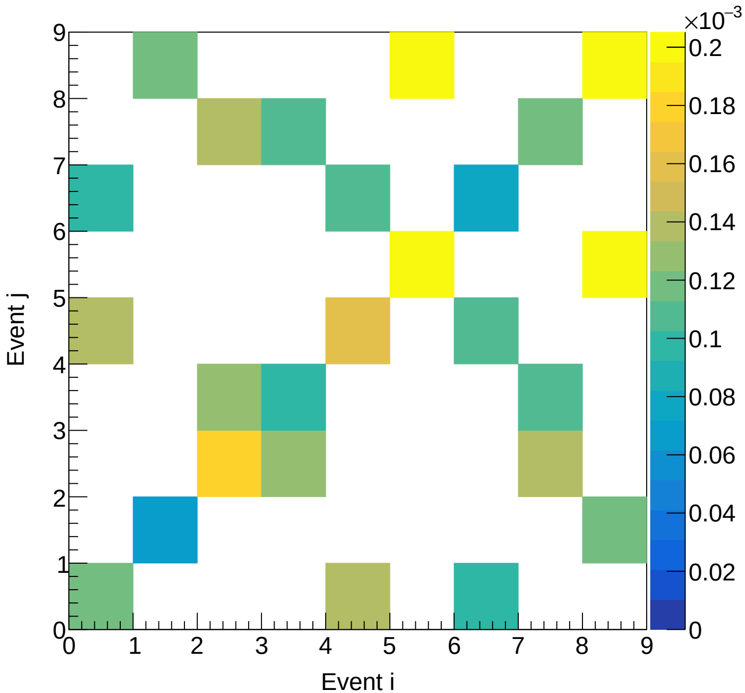
LH2 (total) Covariance | M: [7.5, 8.8) xF: [0.30, 0.35)
