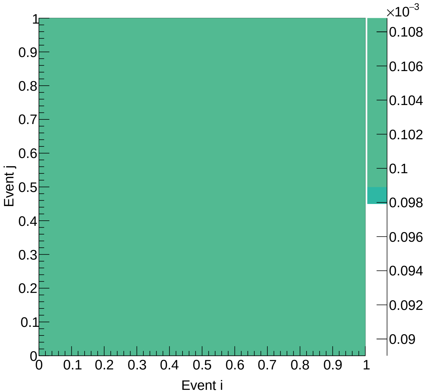
LH2 (total) Covariance | M: [8.8, 10.0) xF: [0.30, 0.35)
