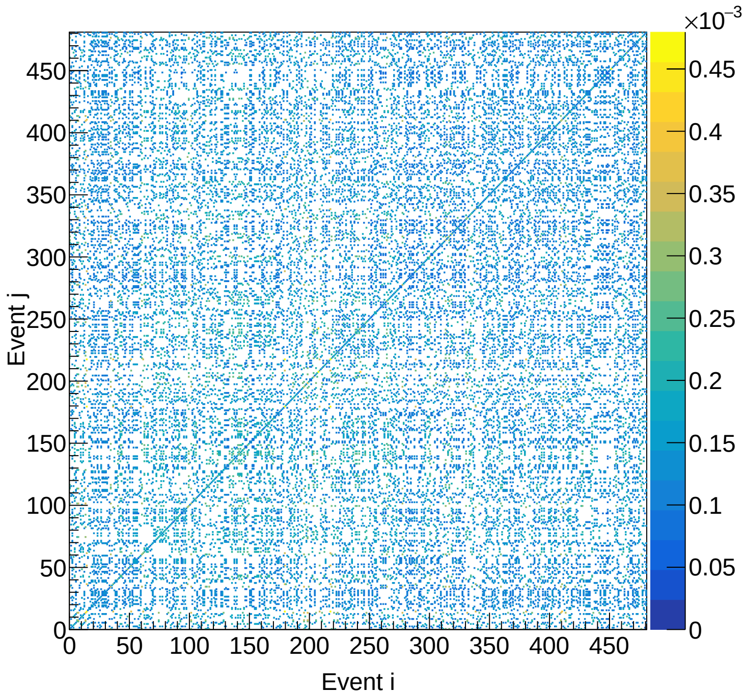
LH2 (total) Covariance | M: [4.5, 4.8) xF: [0.30, 0.35)
