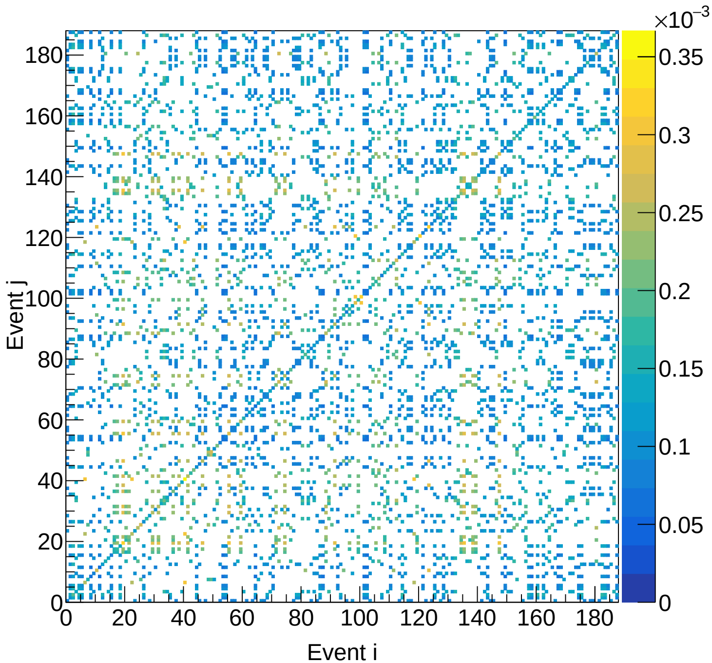
LH2 (total) Covariance | M: [5.4, 5.7) xF: [0.30, 0.35)
