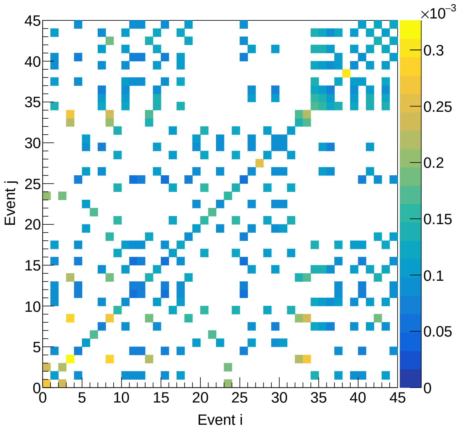
LH2 (total) Covariance | M: [6.3, 6.6] xF: [0.30, 0.35]
