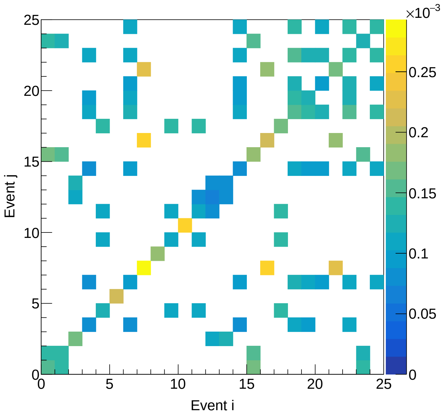
LH2 (total) Covariance | M: [6.6, 6.9) xF: [0.30, 0.35)
