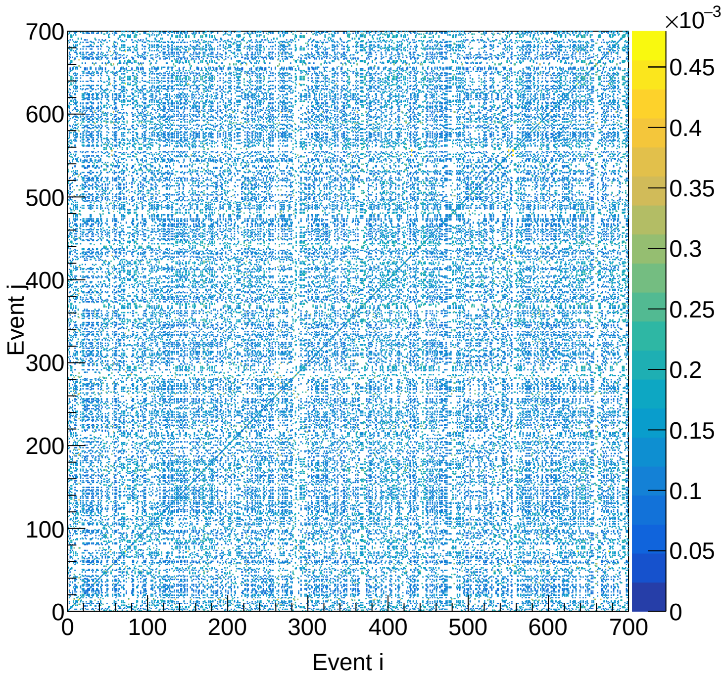
LH2 (total) Covariance | M: [3.9, 4.2) xF: [0.35, 0.40)
