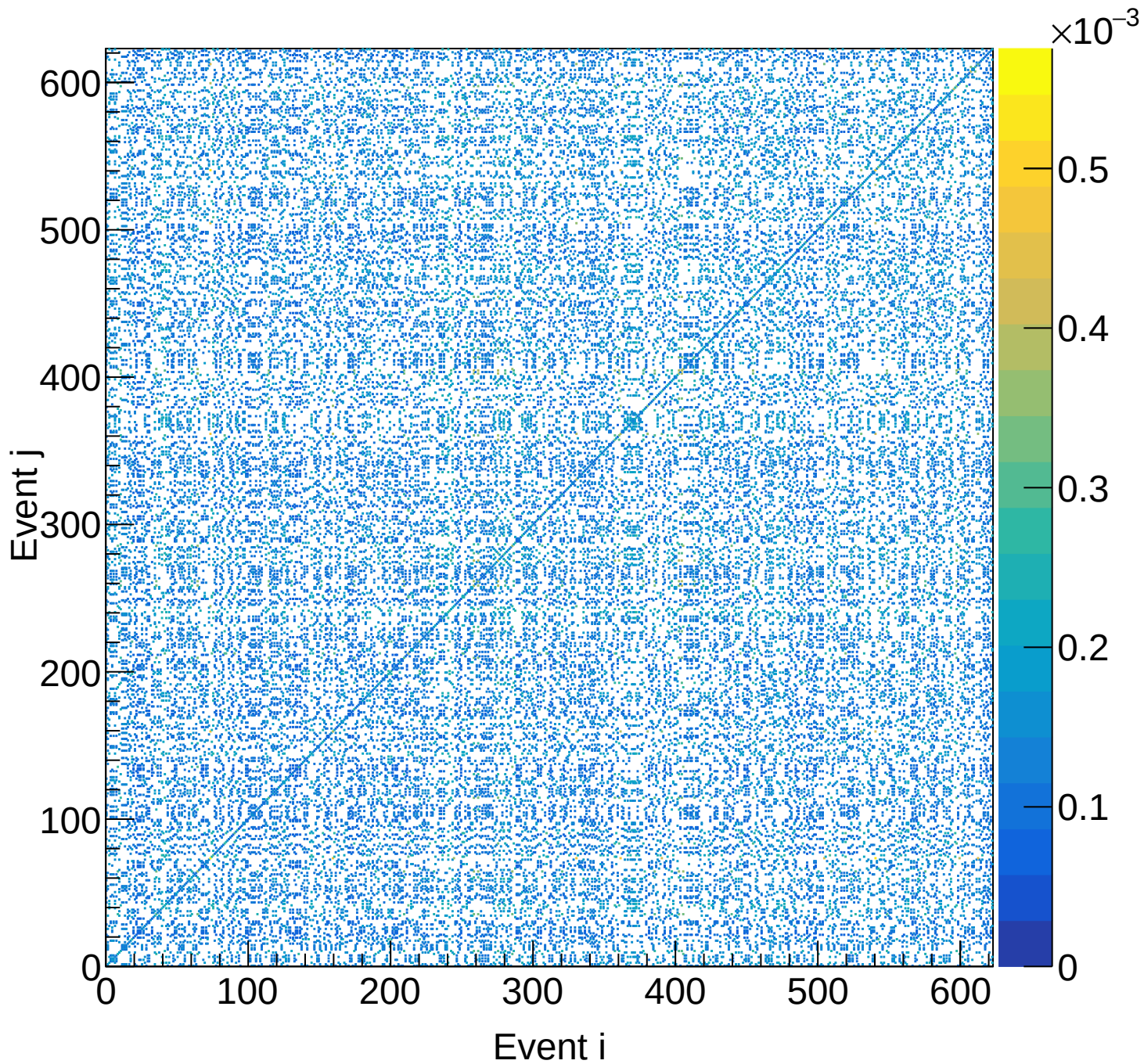
LH2 (total) Covariance | M: [4.2, 4.5) xF: [0.35, 0.40)
