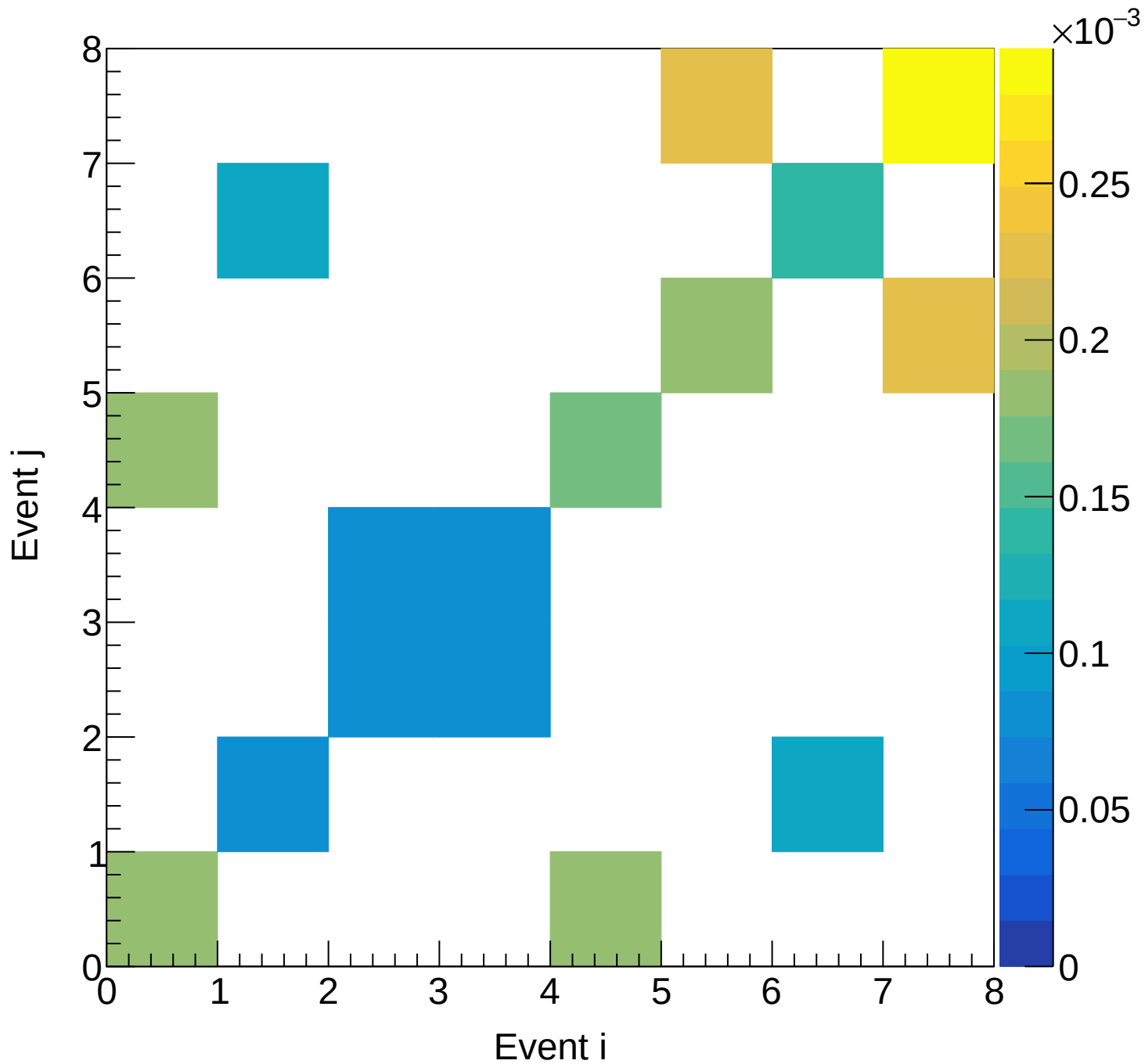
LH2 (total) Covariance | M: [7.5, 8.8) xF: [0.35, 0.40)
