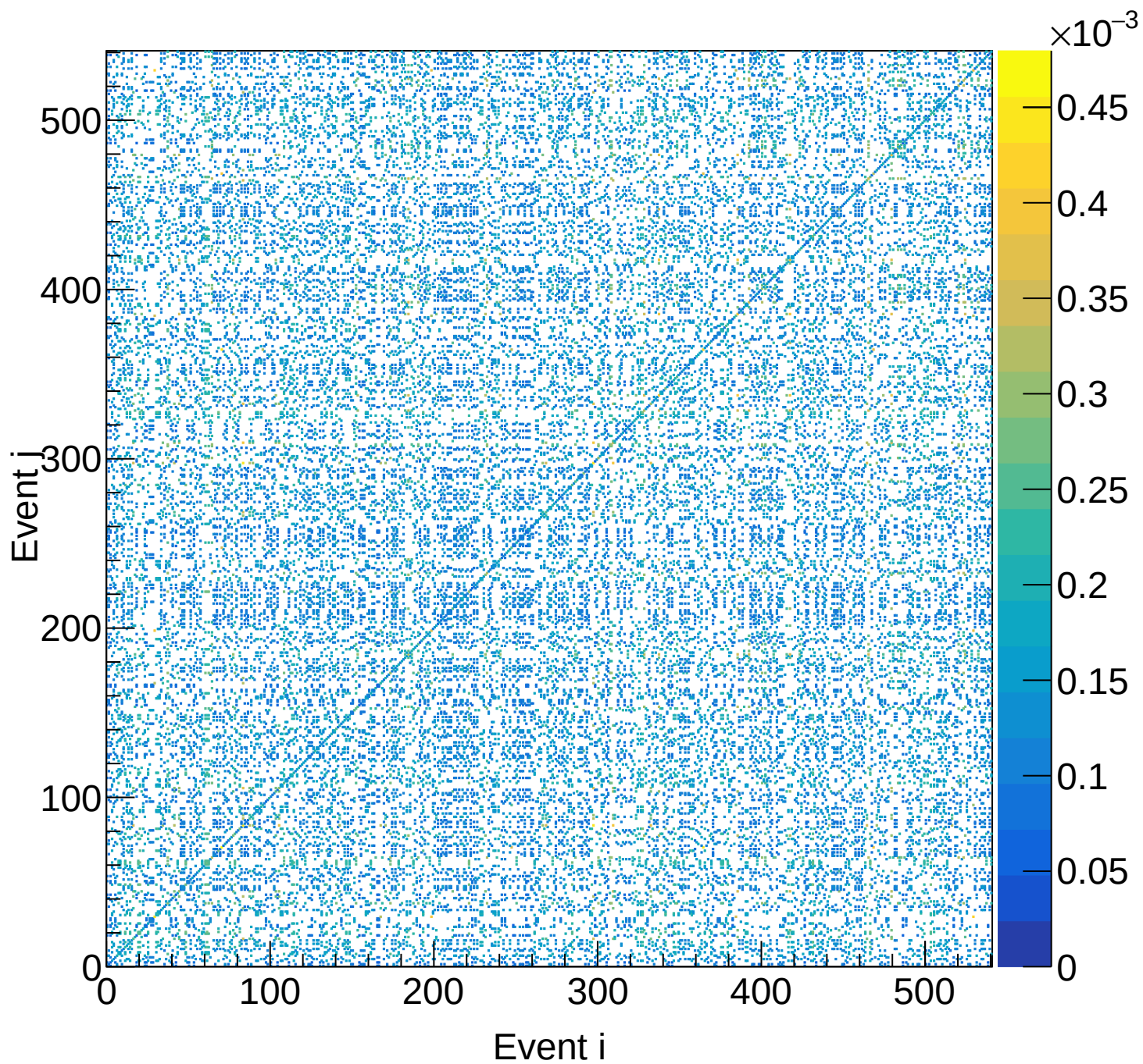
LH2 (total) Covariance | M: [4.5, 4.8) xF: [0.35, 0.40)
