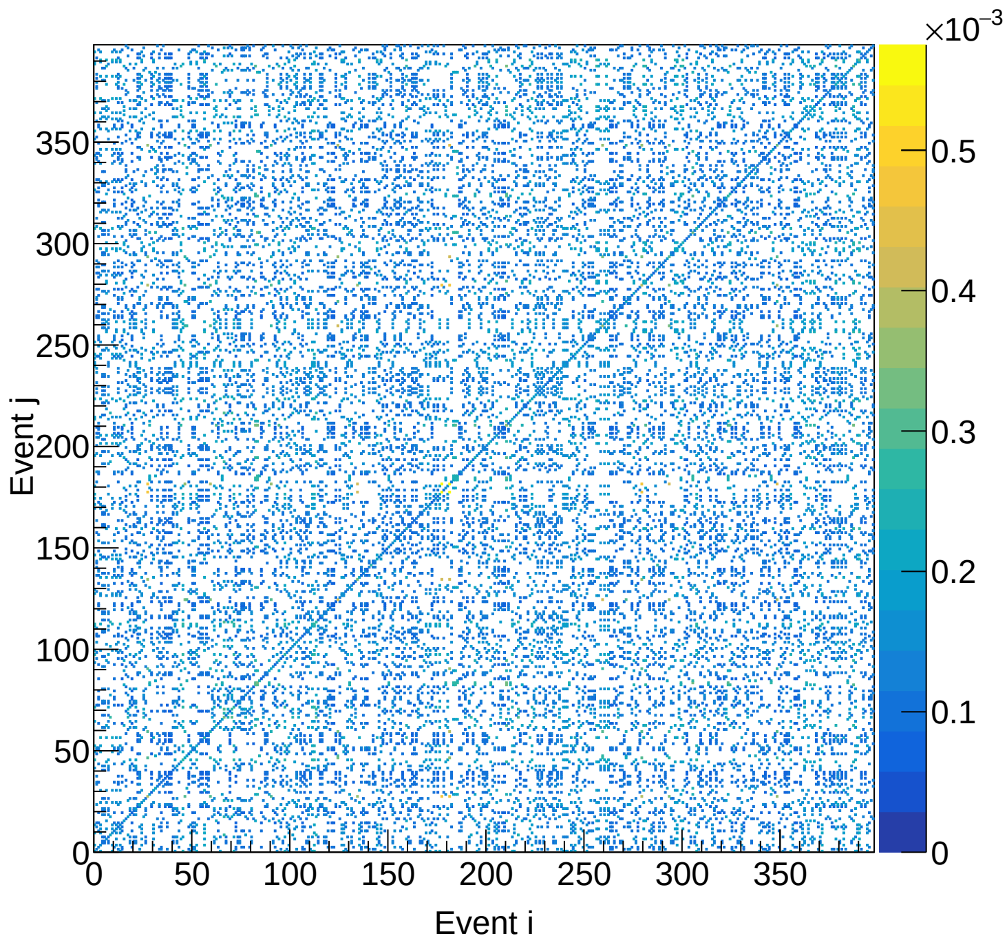
LH2 (total) Covariance | M: [4.8, 5.1) xF: [0.35, 0.40)
