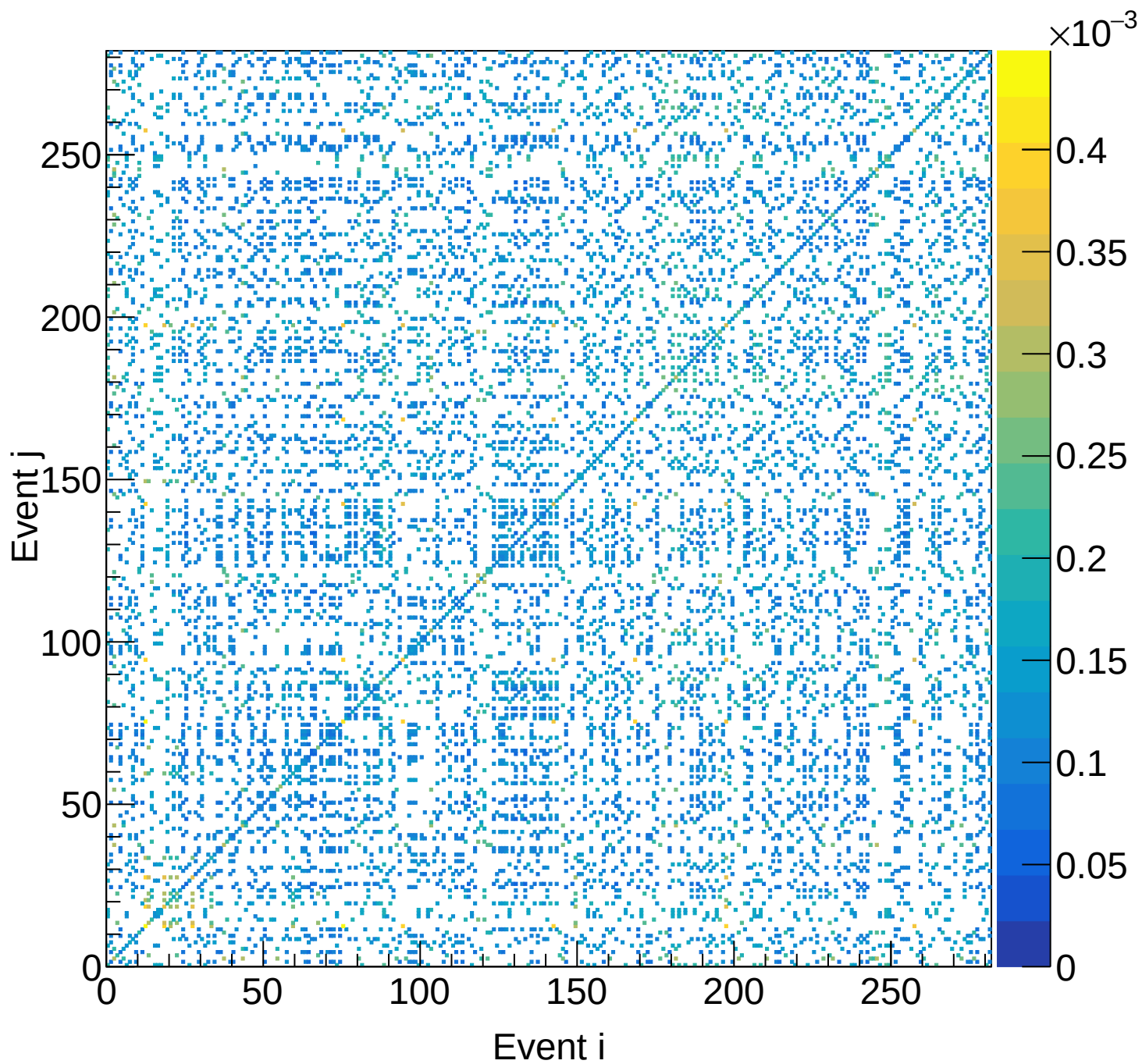
LH2 (total) Covariance | M: [5.1, 5.4) xF: [0.35, 0.40)
