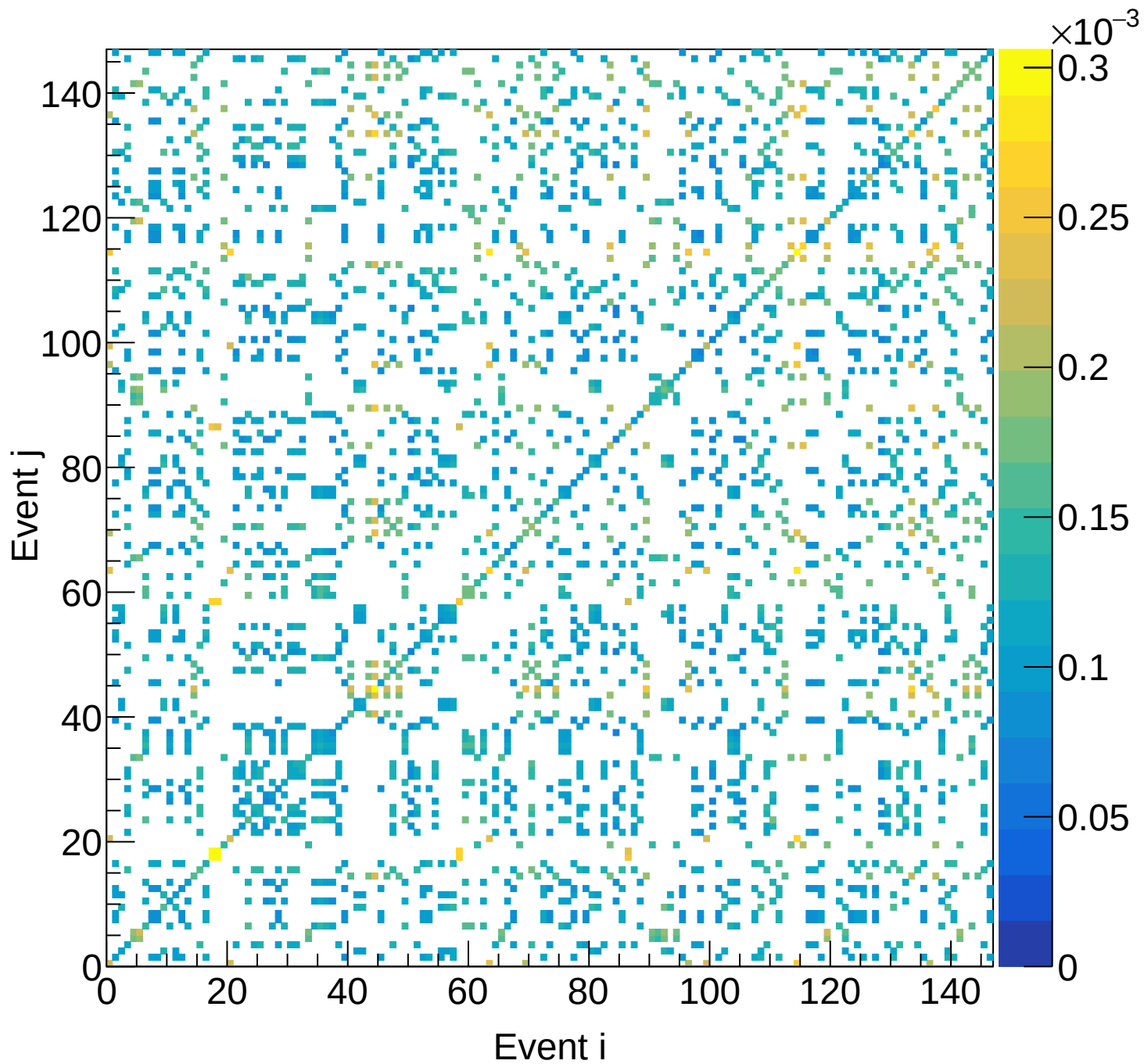
LH2 (total) Covariance | M: [5.4, 5.7) xF: [0.35, 0.40)
