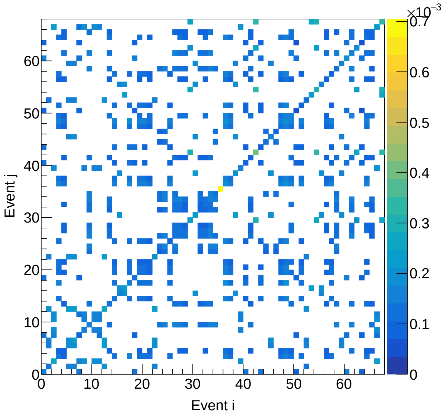
LH2 (total) Covariance | M: [6.0, 6.3) xF: [0.35, 0.40)
