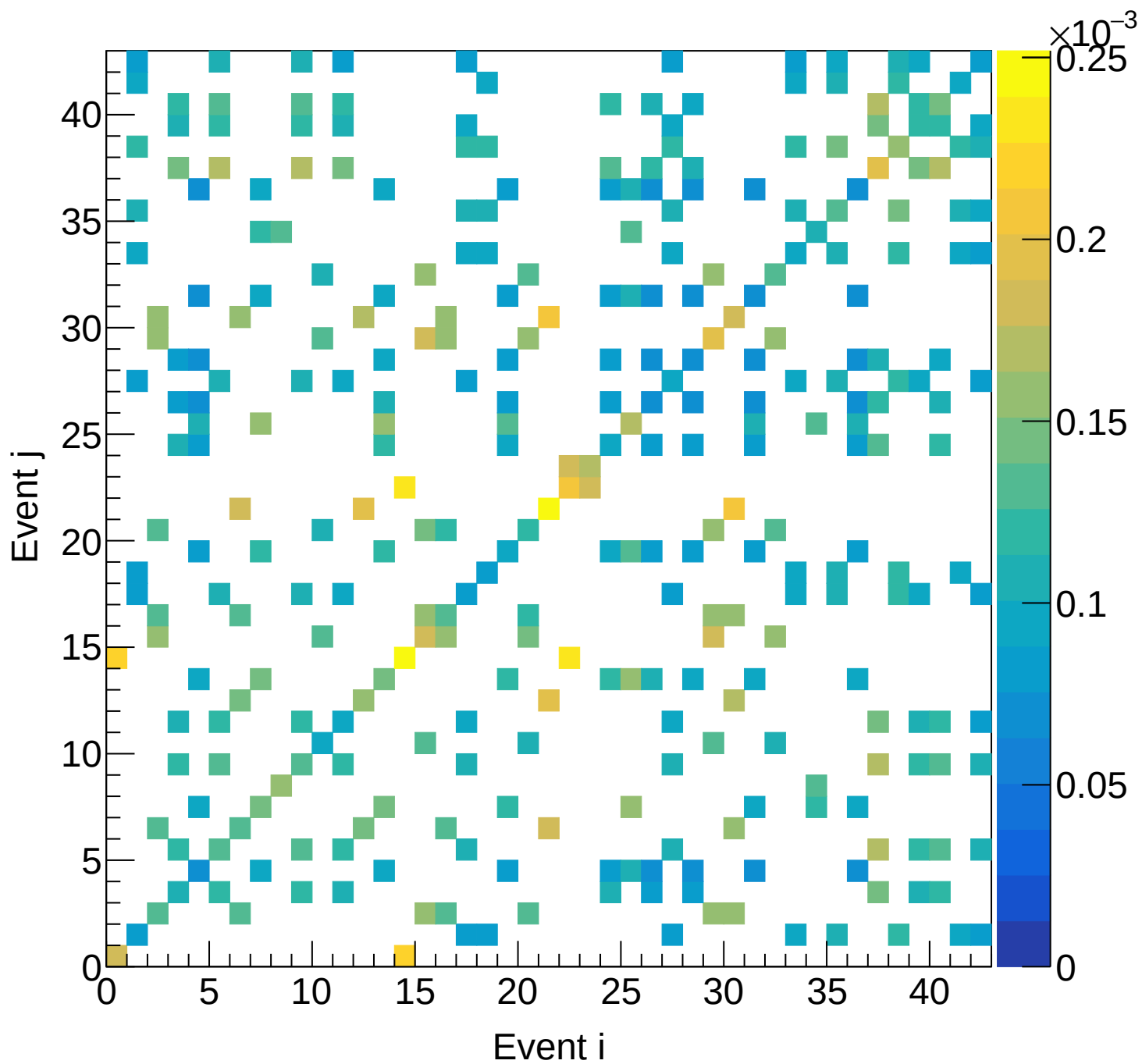
LH2 (total) Covariance | M: [6.3, 6.6) xF: [0.35, 0.40)
