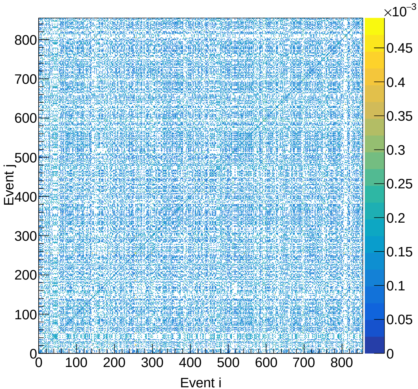
LH2 (total) Covariance | M: [3.9, 4.2) xF: [0.40, 0.45)
