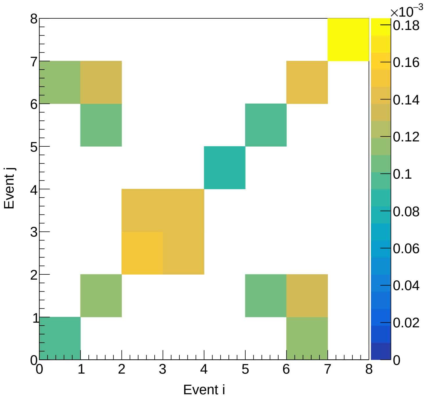
LH2 (total) Covariance | M: [7.5, 8.8) xF: [0.40, 0.45)
