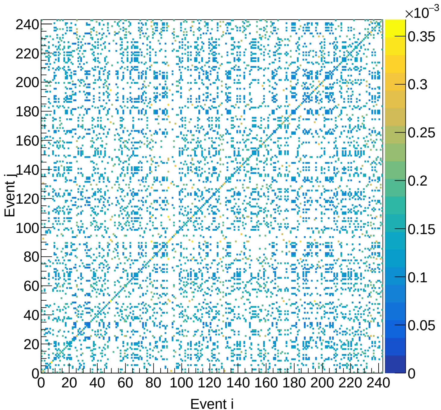
LH2 (total) Covariance | M: [5.1, 5.4) xF: [0.40, 0.45)
