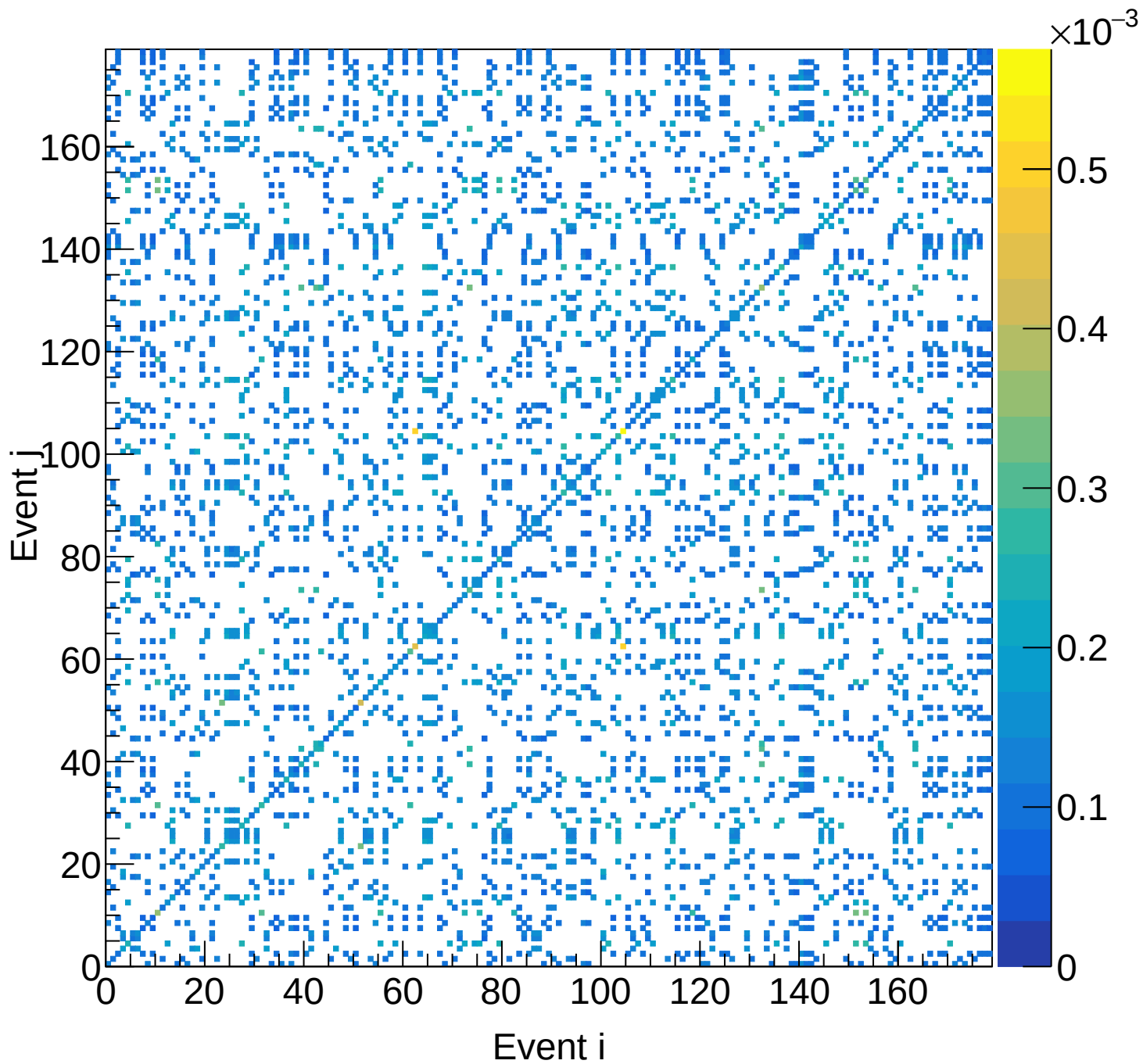
LH2 (total) Covariance | M: [5.4, 5.7) xF: [0.40, 0.45)
