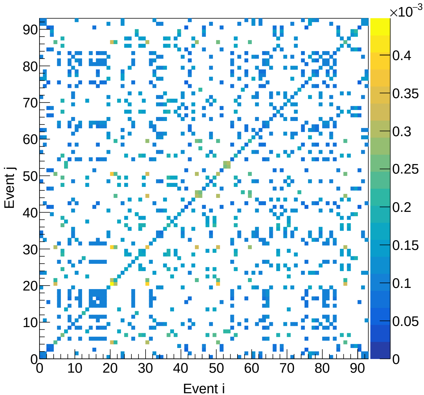
LH2 (total) Covariance | M: [5.7, 6.0] xF: [0.40, 0.45)
