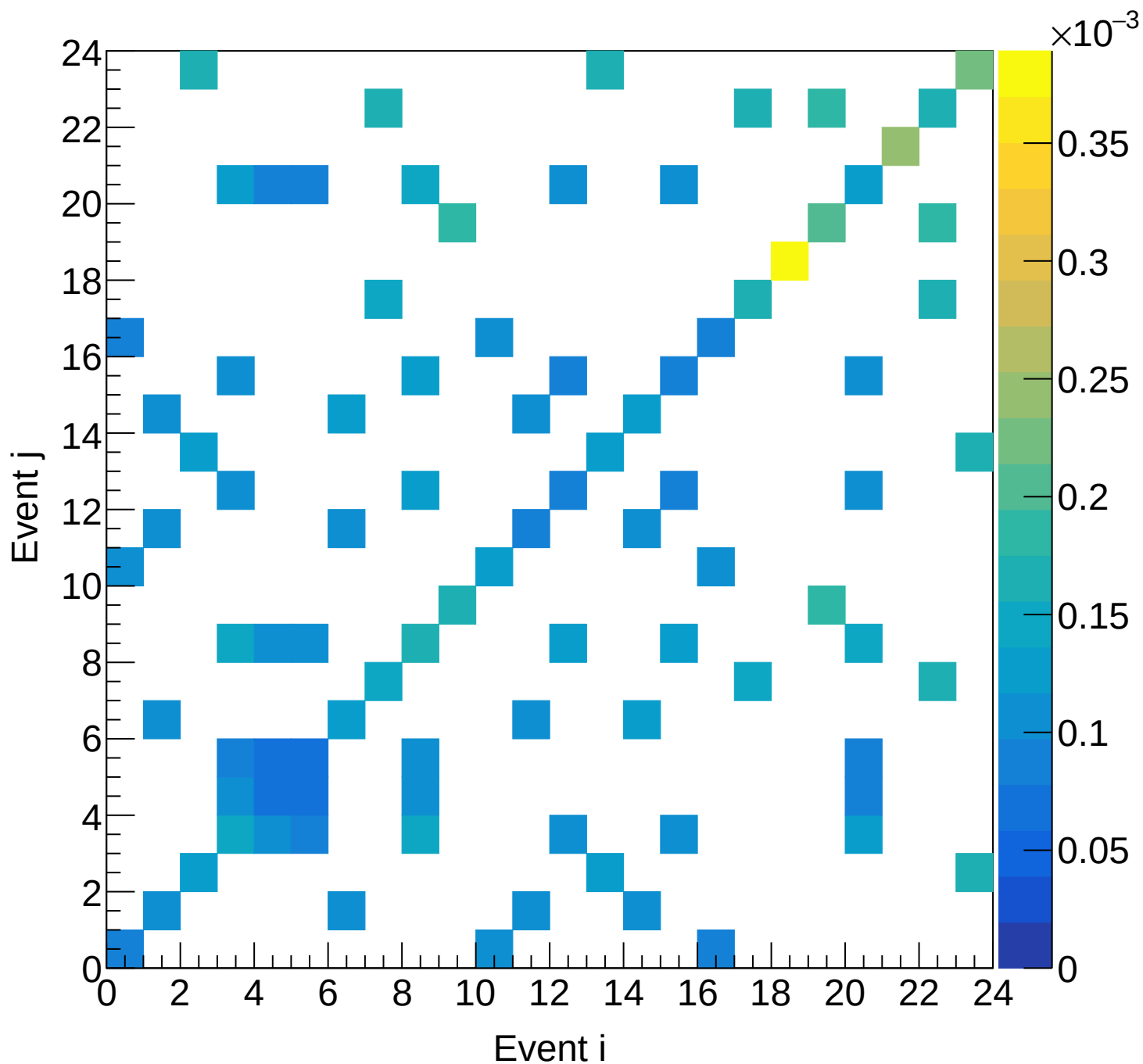
LH2 (total) Covariance | M: [6.6, 6.9) xF: [0.40, 0.45)
