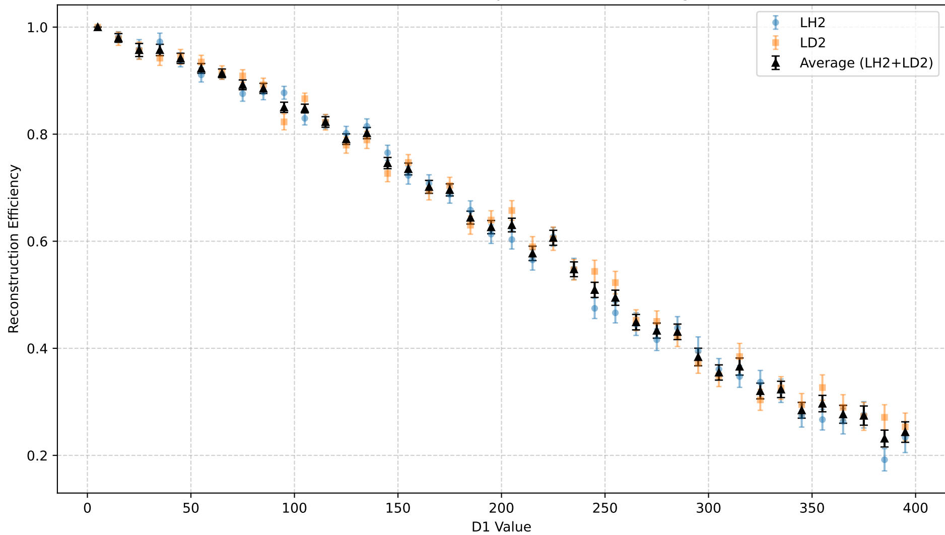
Reconstruction Efficiency: LH2 vs LD2 vs Average
