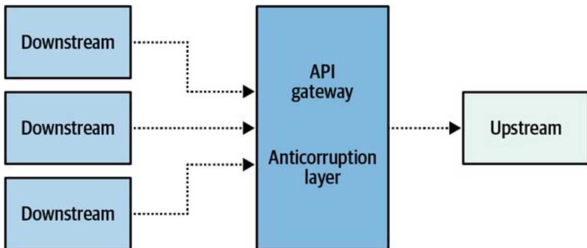
Figure 9-4. Shared anticorruption layer
