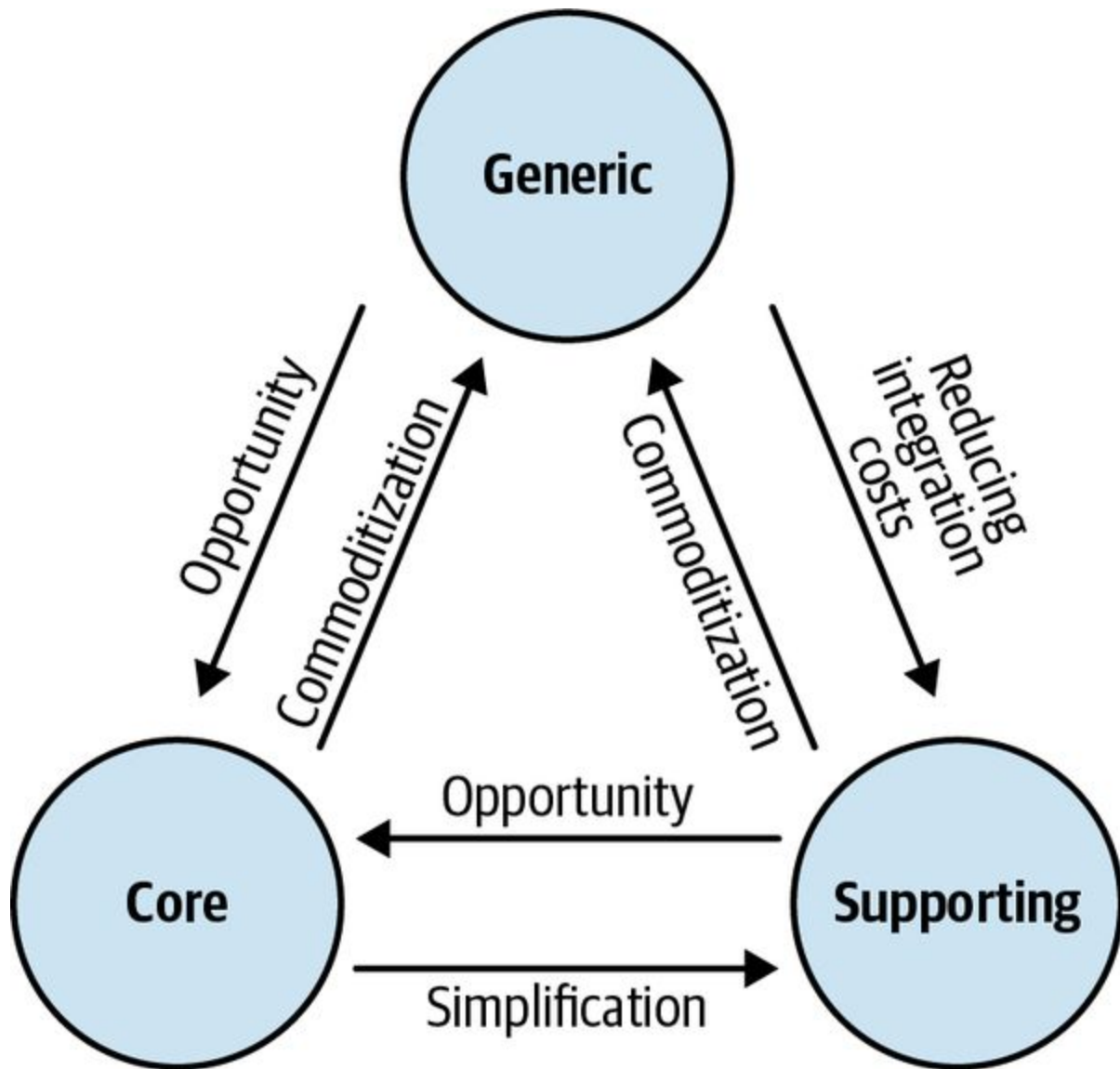
Figure 11-1. Subdomain type change factors
