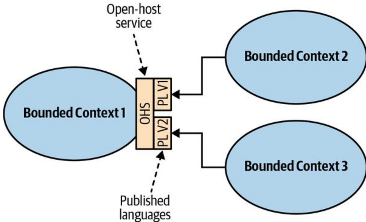
Figure 4-7. Open-host service exposing multiple versions of the published language
