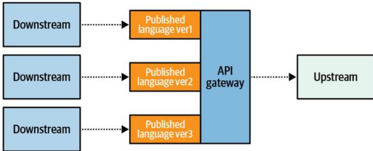
Figure 9-3. Exposing different versions of the published language
