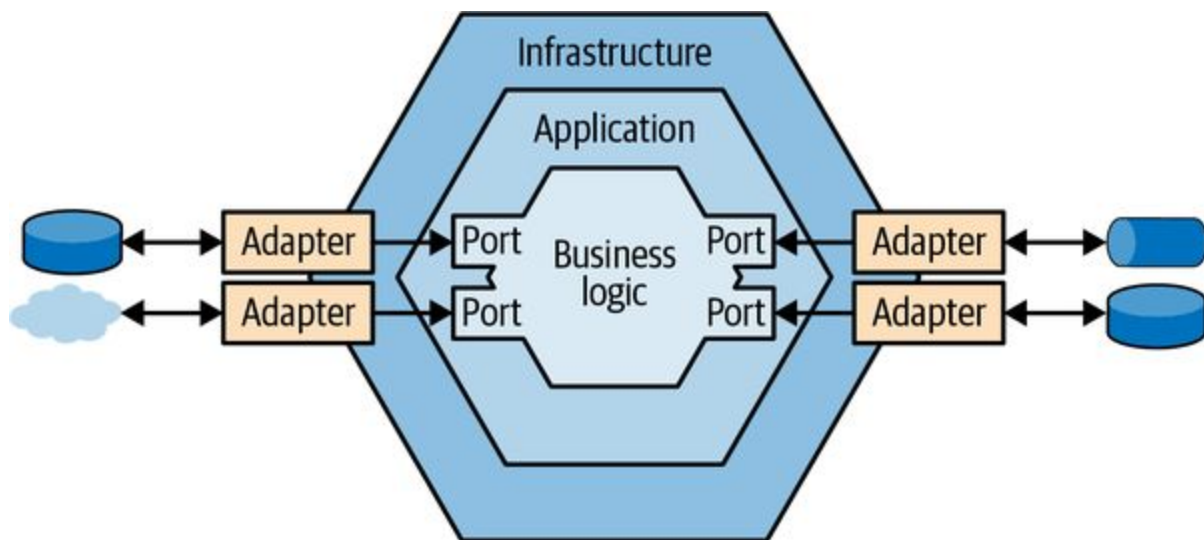
Figure 8-11. Ports & adapters architecture
