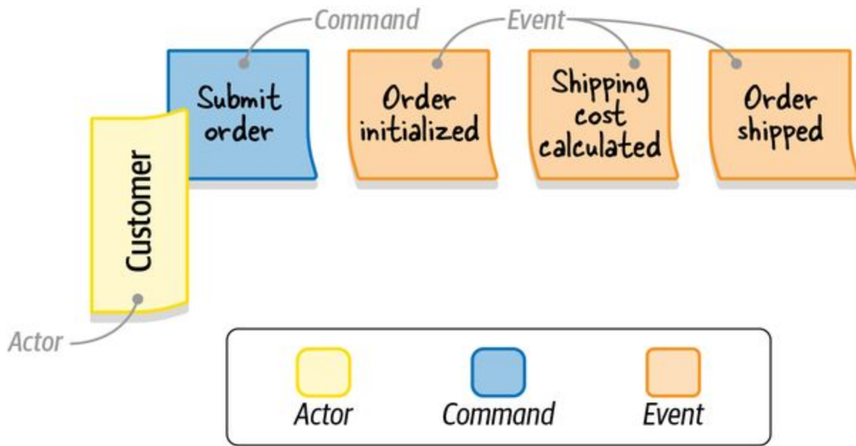
Figure 12-6. The “Submit Order” command, executed by the customer (actor) and followed by the “Order initialized,” “Shipping cost calculated,” and “Order shipped” events
