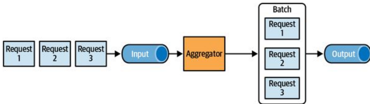
Figure 9-8. Unifying incoming events
