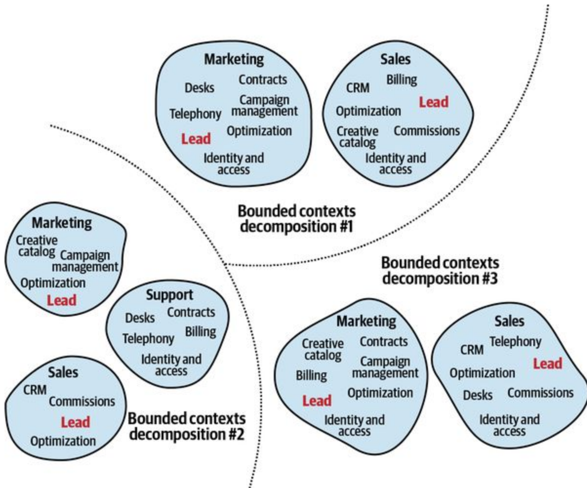
Figure 14-9. Alternative decompositions to bounded contexts
