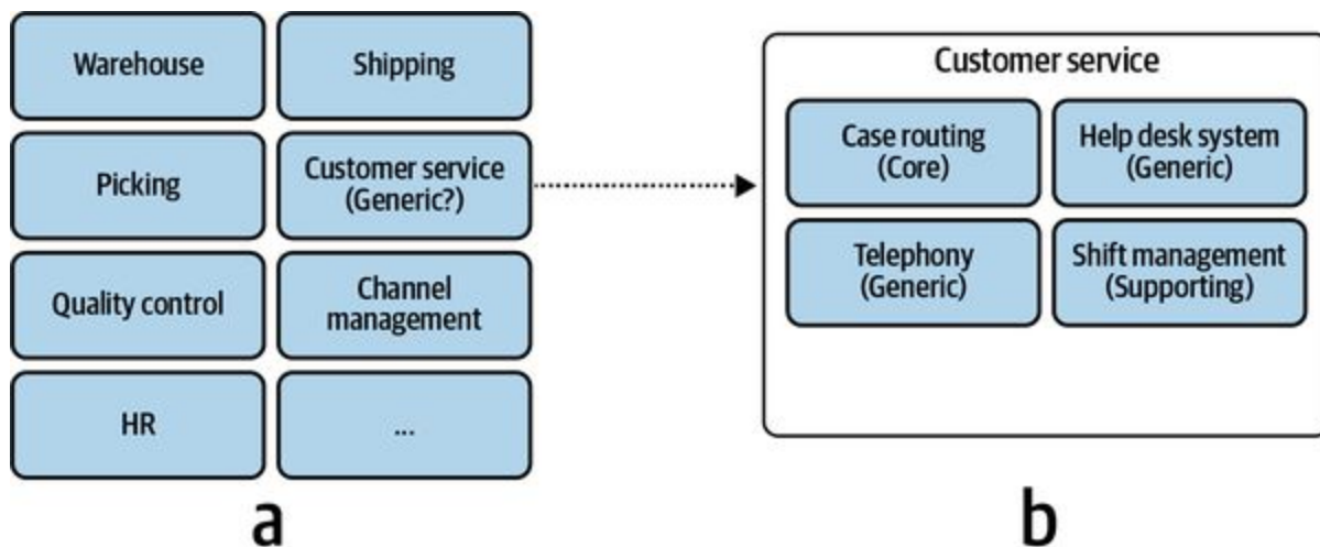
Figure 1-2. Analyzing the inner workings of a suspectedly generic subdomain to find the finer-grained core subdomain, supporting subdomain, and two generic subdomains
