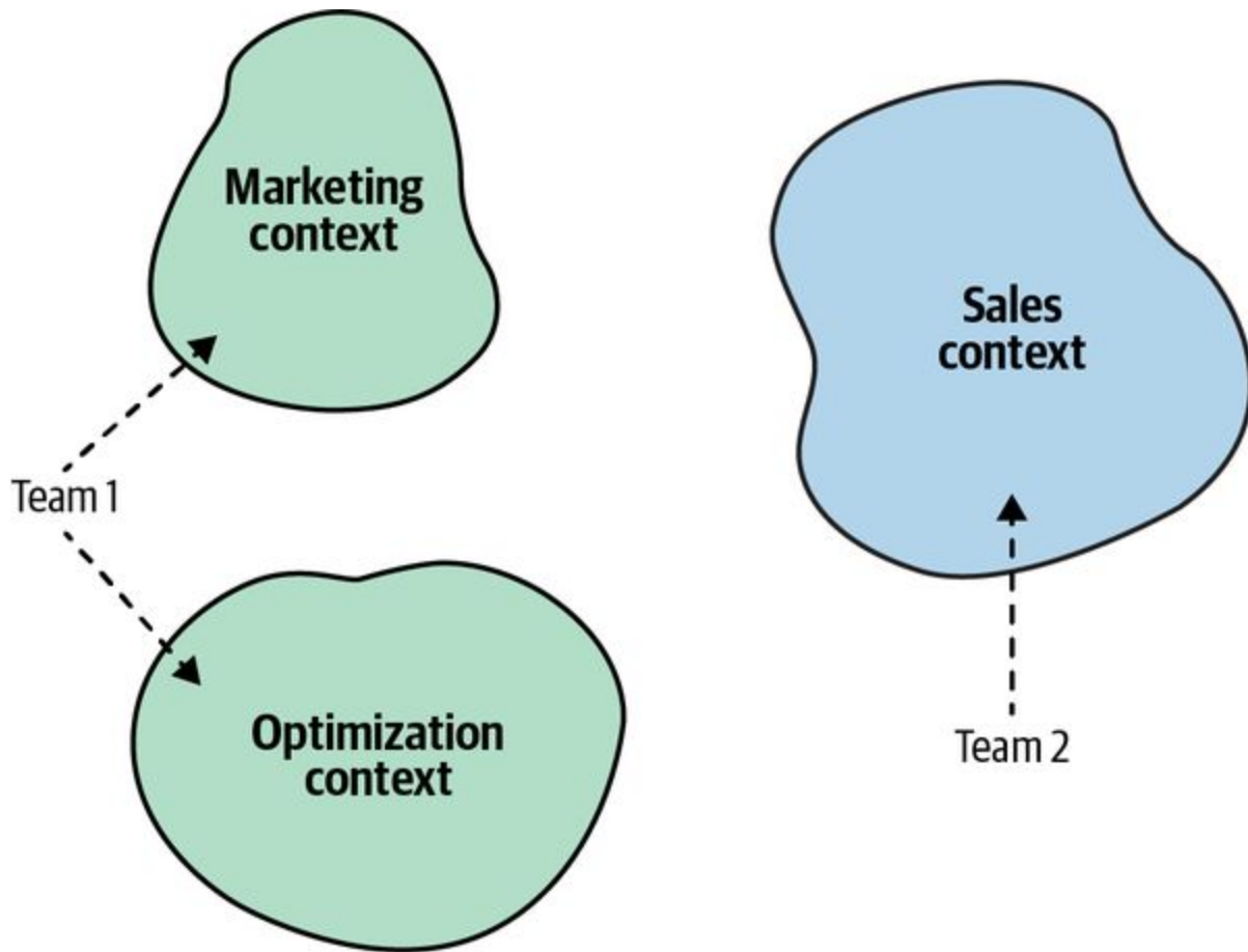
Figure 3-8. Team 1 working on the Marketing and Optimization bounded contexts, while Team 2 works on the Sales bounded context
