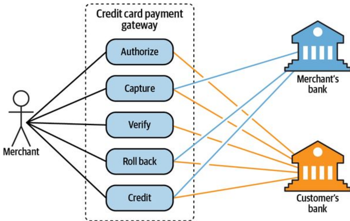
Figure 1-3. Use case diagram of a credit card payment subdomain
