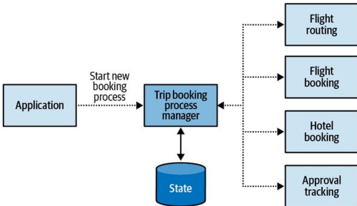
Figure 9-15. Trip booking process manager
