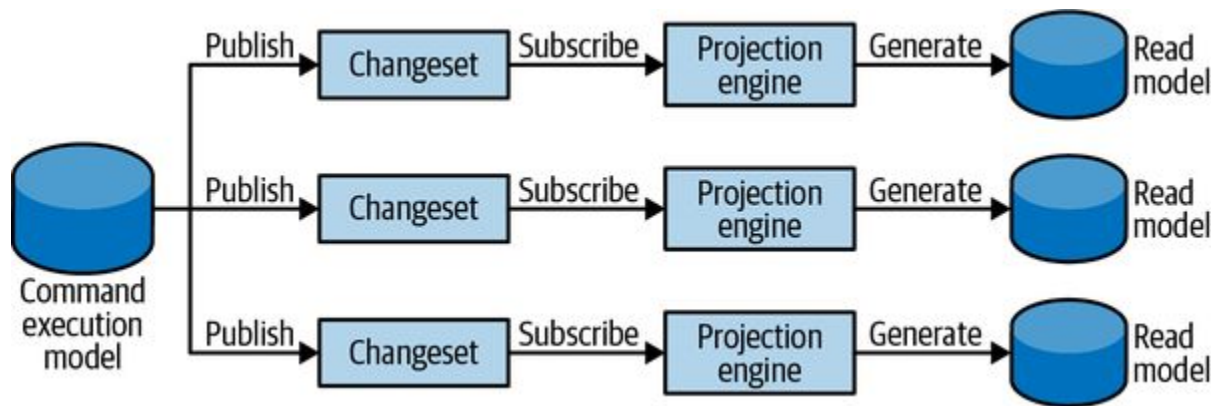
Figure 8-16. Asynchronous projection of read models
