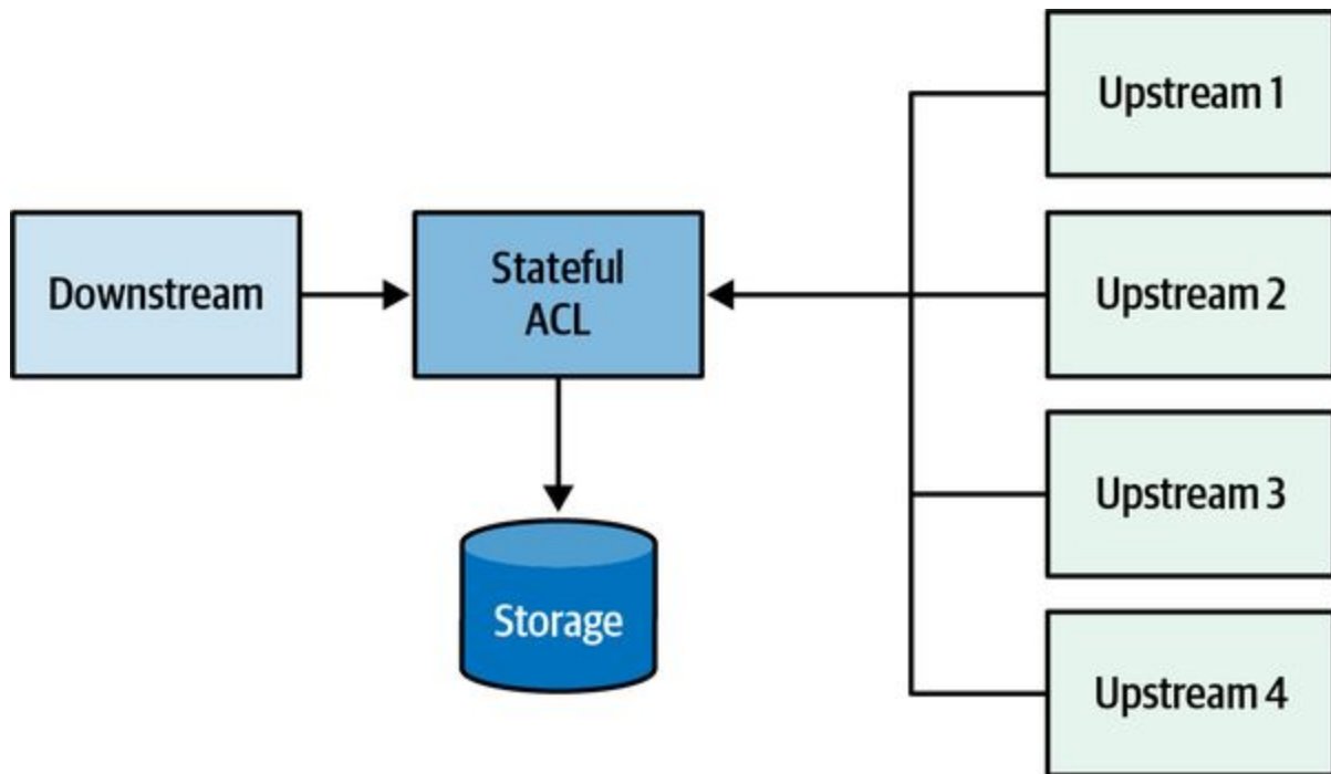
Figure 9-10. Simplifying the integration model using the anticorruption layer pattern
