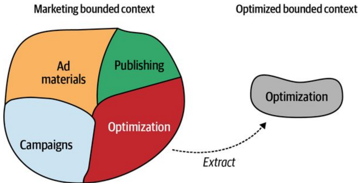
Figure 13-2. Extracting a bounded context by turning a logical boundary into a physical boundary
