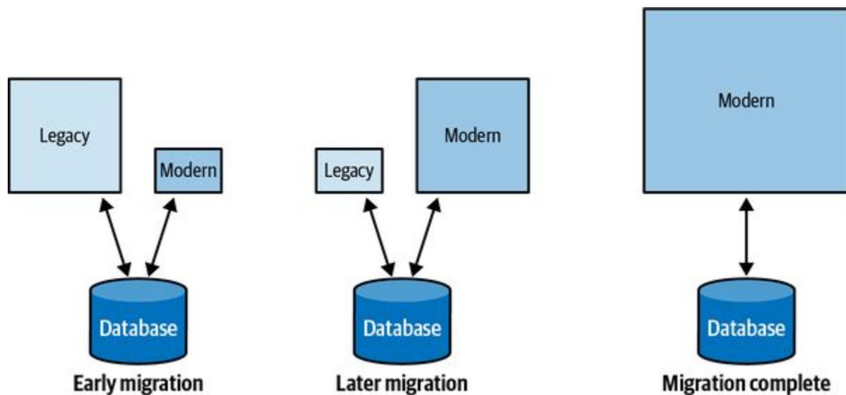
Figure 13-5. Both the legacy and the modernized systems temporarily working with the same database
