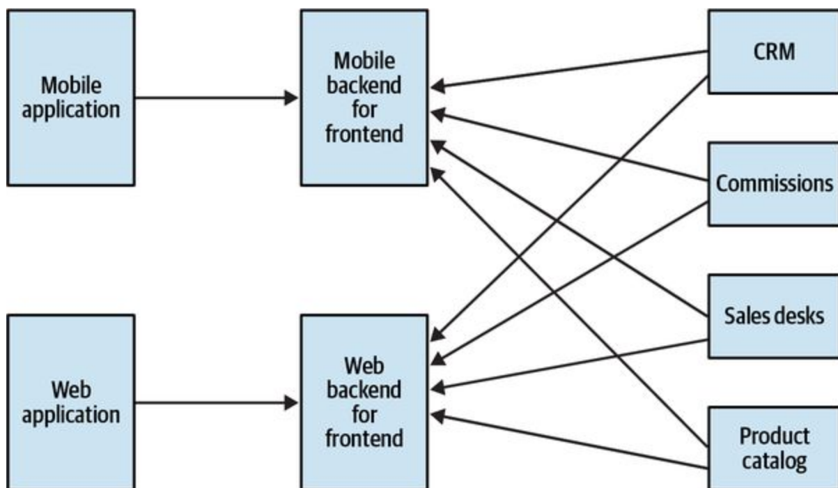
Figure 15-4. Backend for frontend
