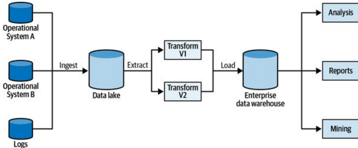
Figure 16-11. Multiple versions of the same ETL script accommodating different versions of the operational model
