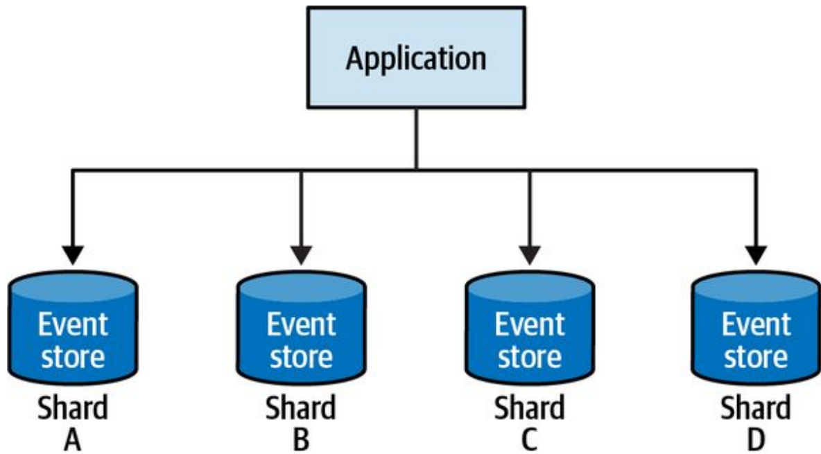
Figure 7-3. Sharding the event store
