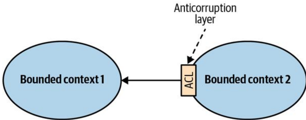
Figure 4-5. Integration through an anticorruption layer
