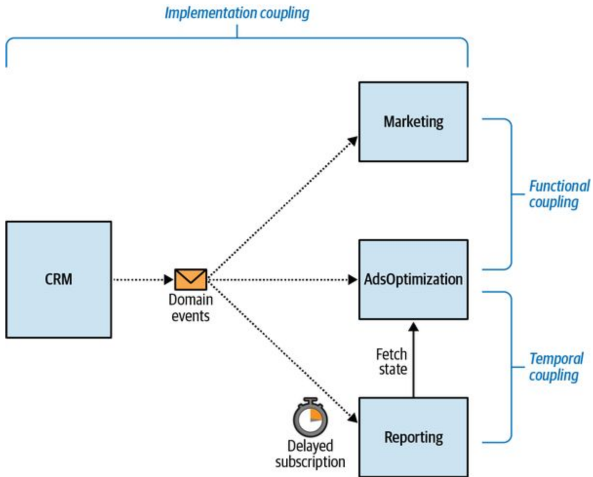
Figure 15-5. Strongly coupled distributed system
