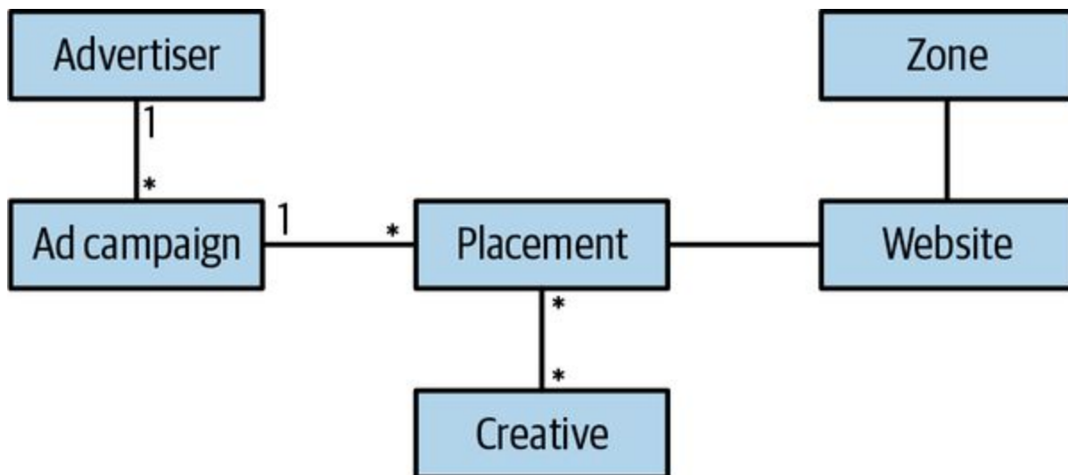
Figure 5-4. A more complicated data model with one-to-many and many-to-many relationships
