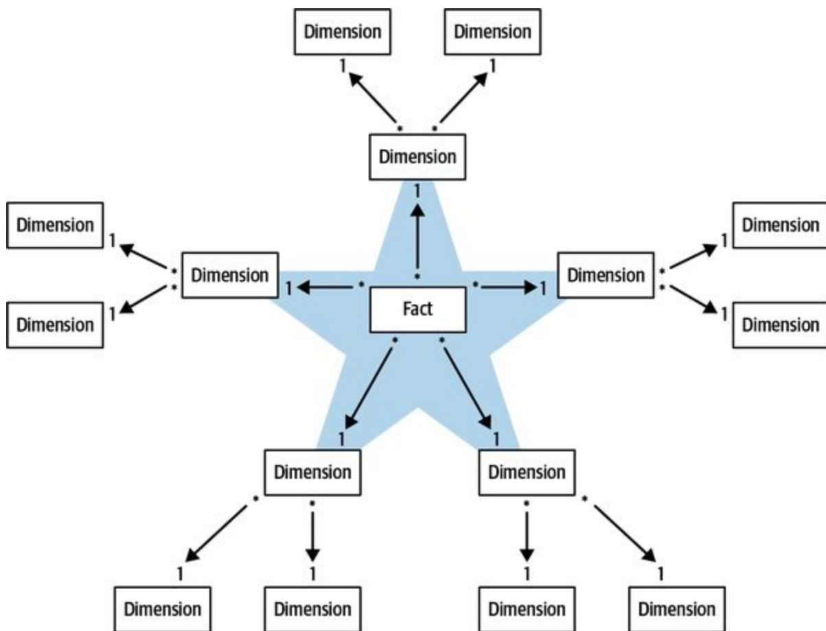
Figure 16-6. Multilevel dimensions in the snowflake schema
