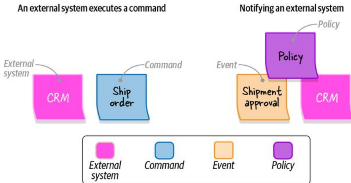
Figure 12-9. External system triggering execution of a command (left) and approval of the event being communicated to the external system (right)
