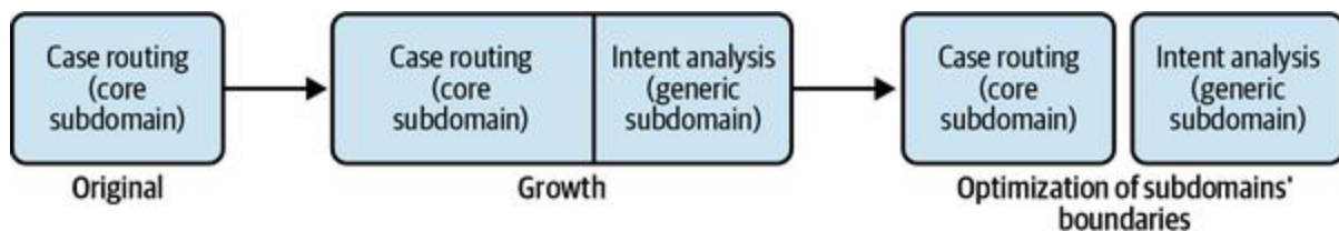
Figure 11-3. Optimizing subdomains' boundaries to accommodate growth
