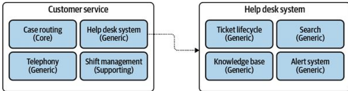
Figure 1-4. Distilling the help desk system subdomain, revealing generic inner components
