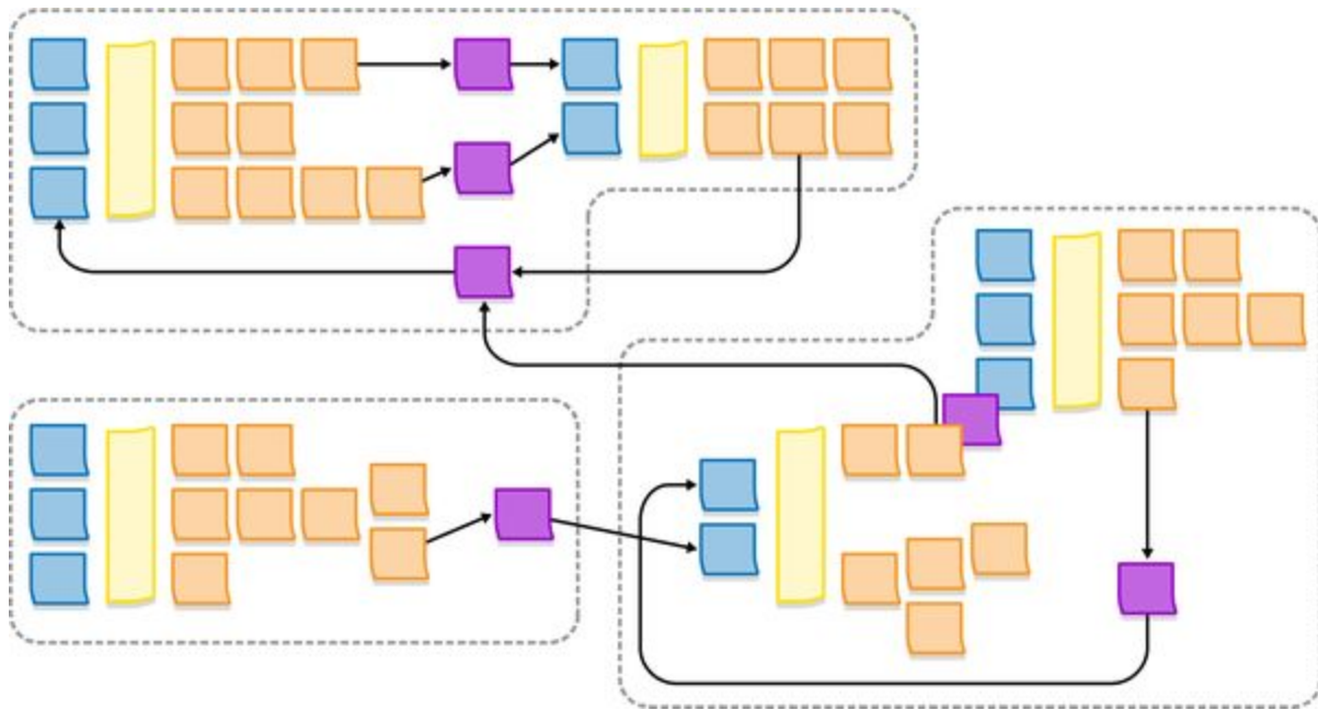
Figure 12-11. A possible decomposition of the resultant system into bounded contexts
