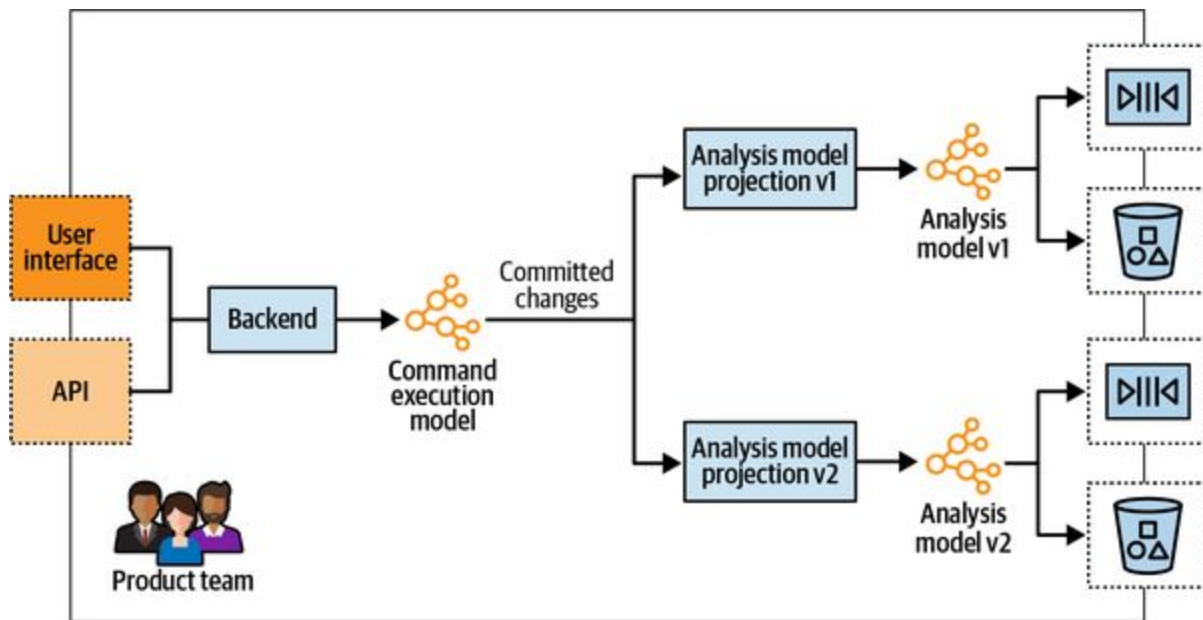
Figure 16-15. Leveraging the CQRS pattern to simultaneously serve the analytical data in two different schema versions
