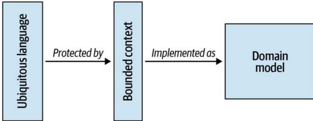
Figure A-3. Introduction of strategic design concepts into our understanding of domain-driven design
