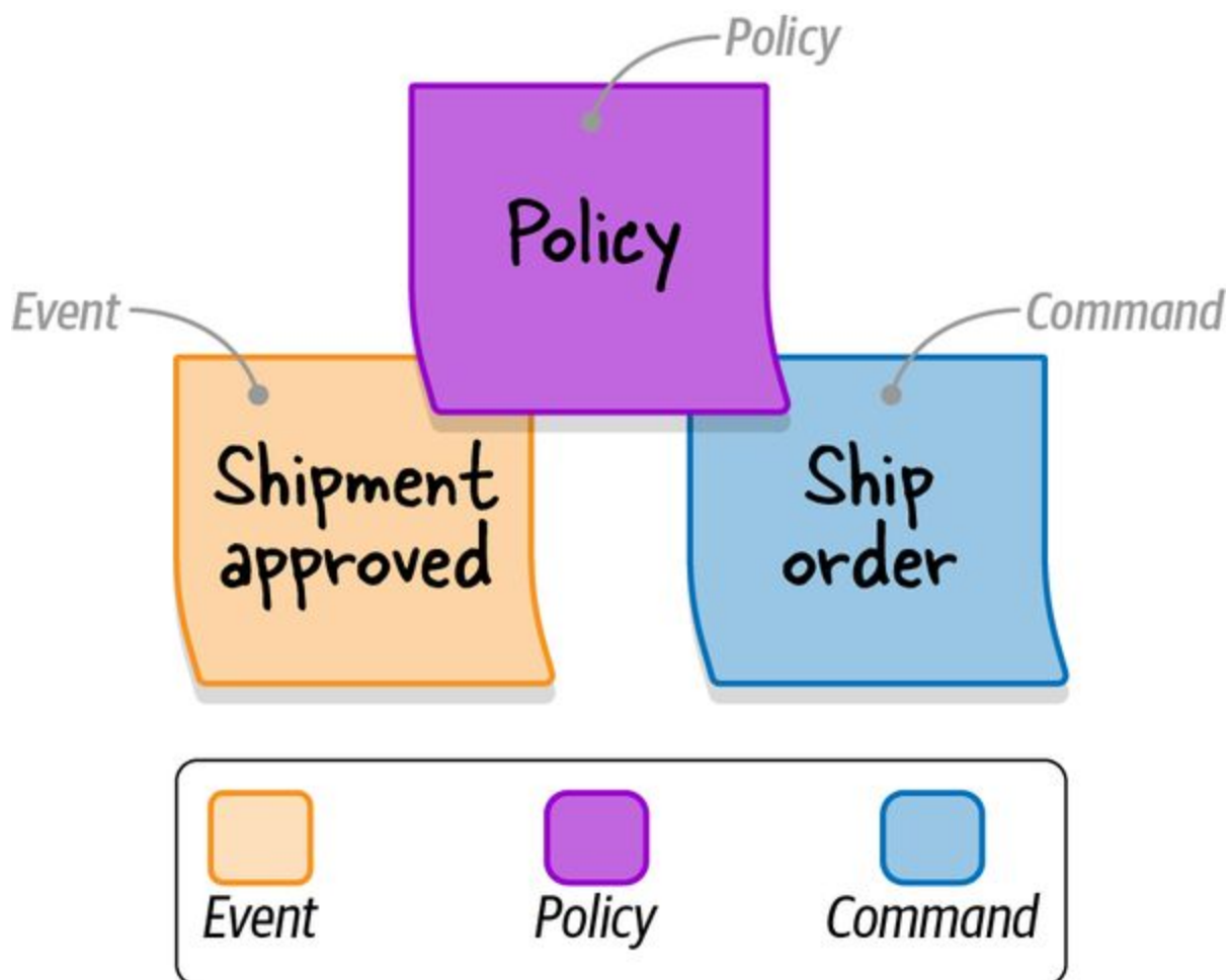
Figure 12-7. An automation policy that triggers the “Ship Order” command when the “Shipment Approved” event is observed
