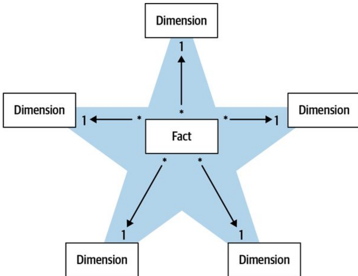
Figure 16-5. The many-to-one relationship between facts and their dimensions
