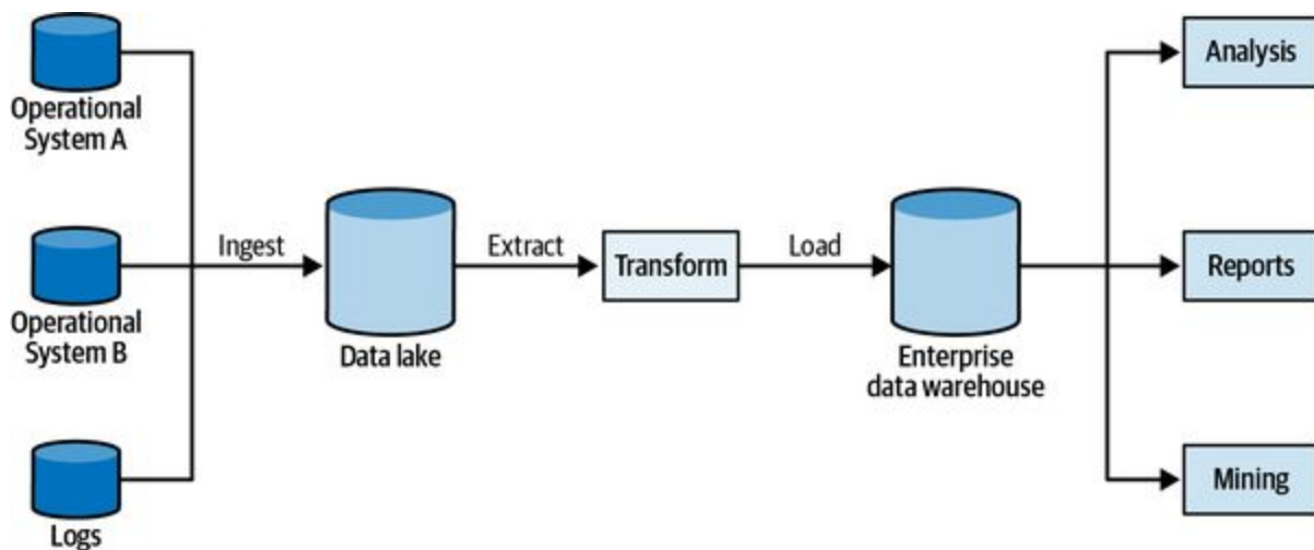
Figure 16-10. Data lake architecture
