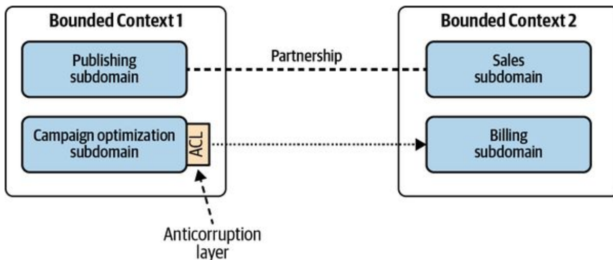
Figure 4-9. Complicated context map
