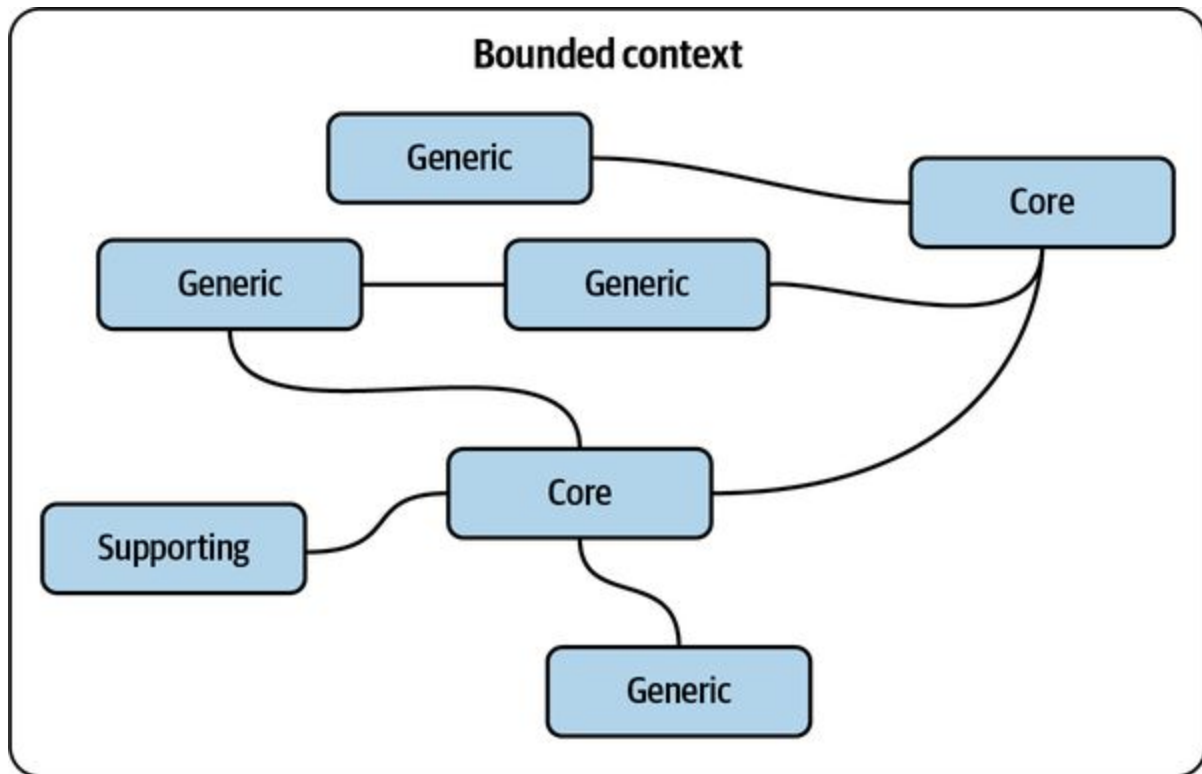
Figure 10-2. Wide bounded context boundaries
