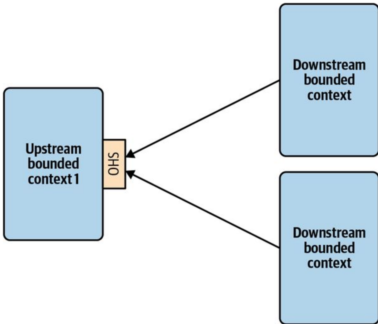
Figure 14-12. Integrating services through a published language
