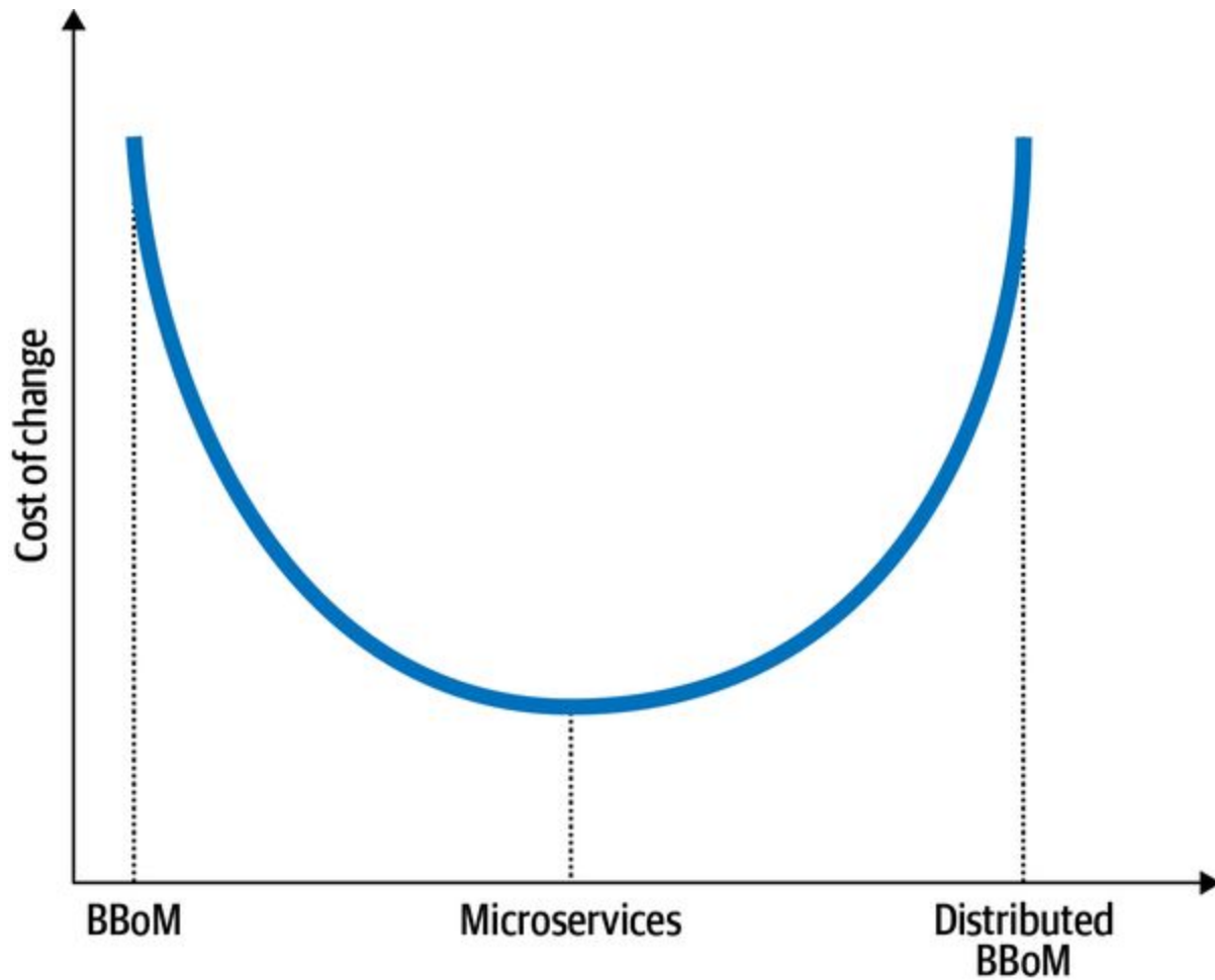
Figure 14-7. Granularity and cost of change
