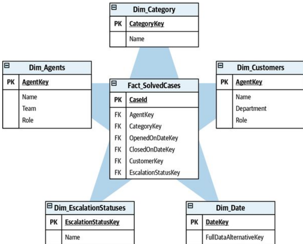
Figure 16-4. The SolvedCases fact surrounded by its dimensions
