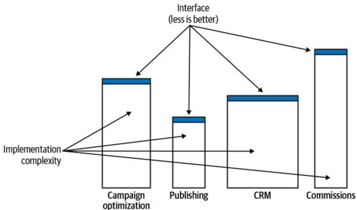
Figure 14-11. Subdomains
