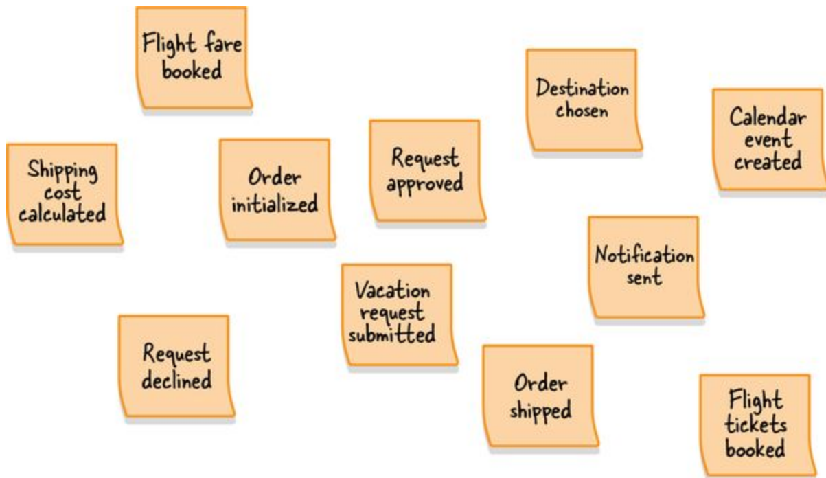
Figure 12-2. Unstructured exploration
