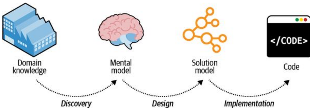
Figure 2-2. Model transformations
