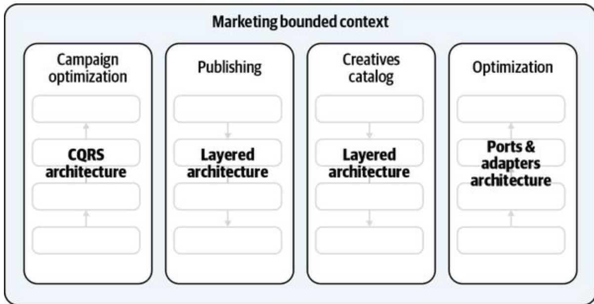
Figure 8-18. Architectural slices
