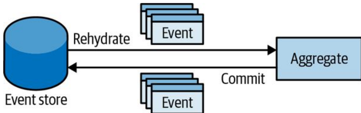
Figure 7-1. Event-sourced aggregate
