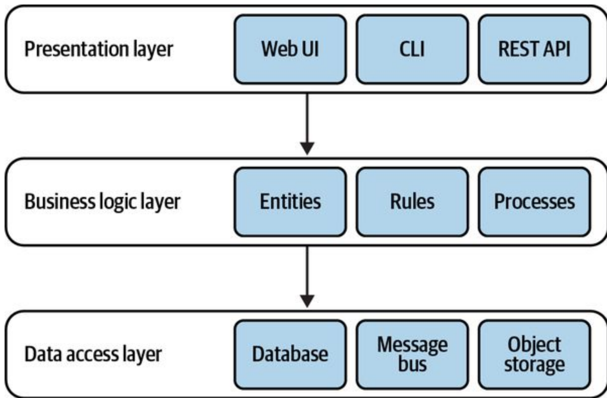
Figure 8-5. Layered architecture
