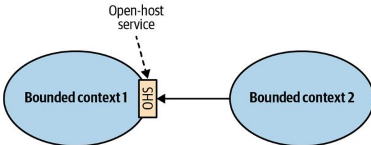
Figure 4-6. Integration through an open-host service
