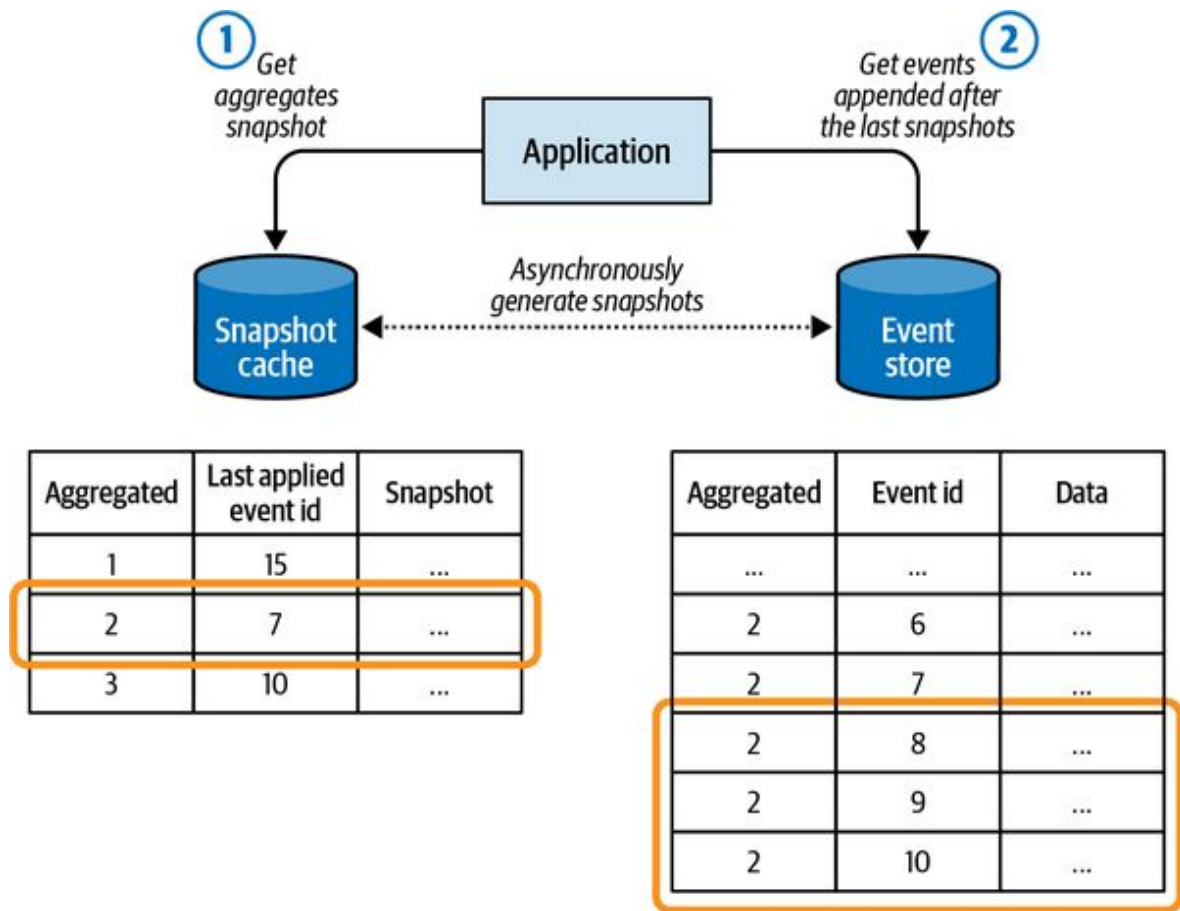
Figure 7-2. Snapshotting an aggregate's events
