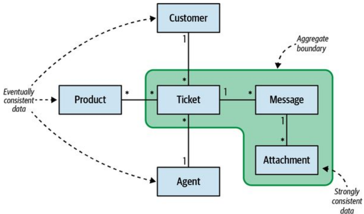
Figure 6-4. Aggregate as consistency boundary
