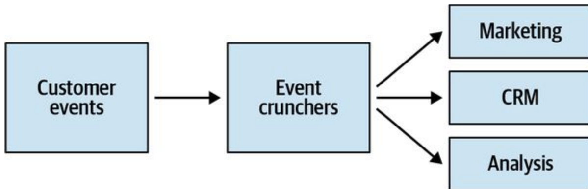
Figure A-4. The event crunchers bounded context handling the incoming customer events
