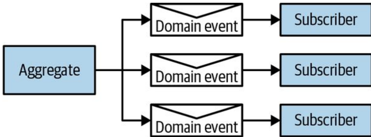
Figure 6-6. Domain events publishing flow
