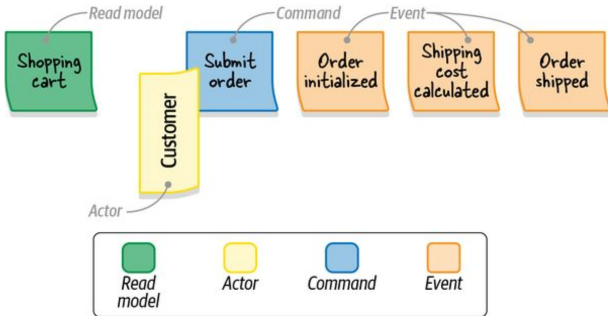
Figure 12-8. The view of the “Shopping cart” (read model) needed for the customer (actor) to make their decision to submit the order (command)
