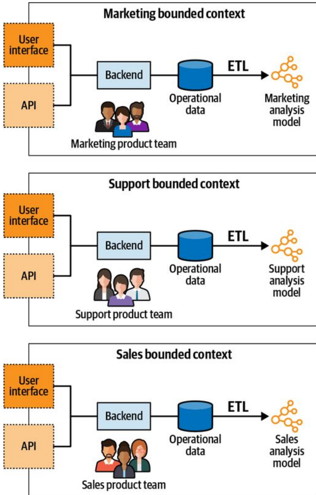
Figure 16-12. Aligning the ownership boundaries of the analytical models with the bounded contexts' boundaries
