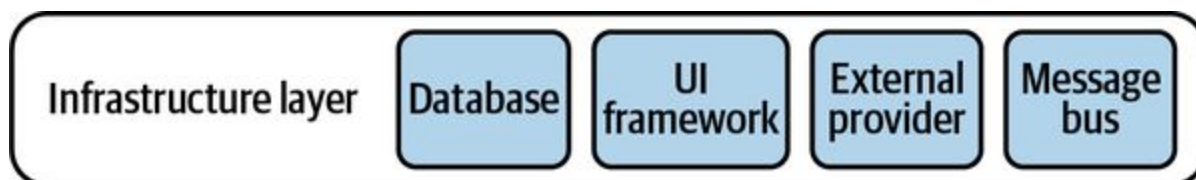
Figure 8-8. Presentation and data access layers combined into an infrastructure layer
