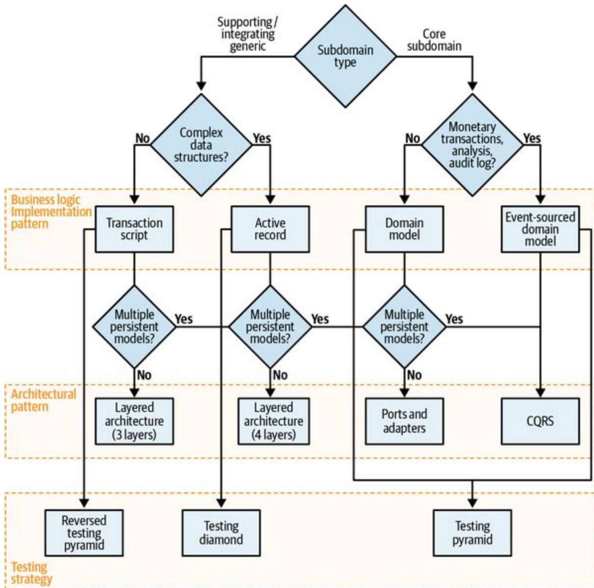
Figure 10-7. Tactical design decision tree
