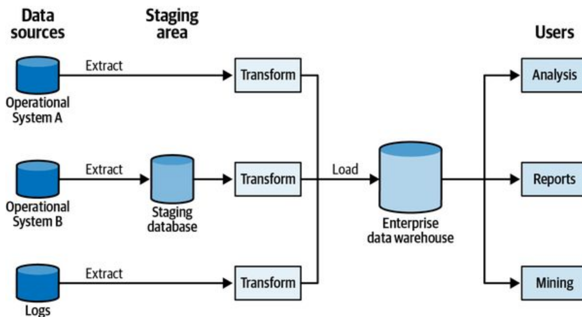
Figure 16-7. A typical enterprise data warehouse architecture
