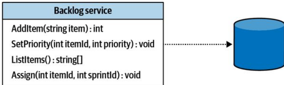
Figure 5-1. Transaction script interface
