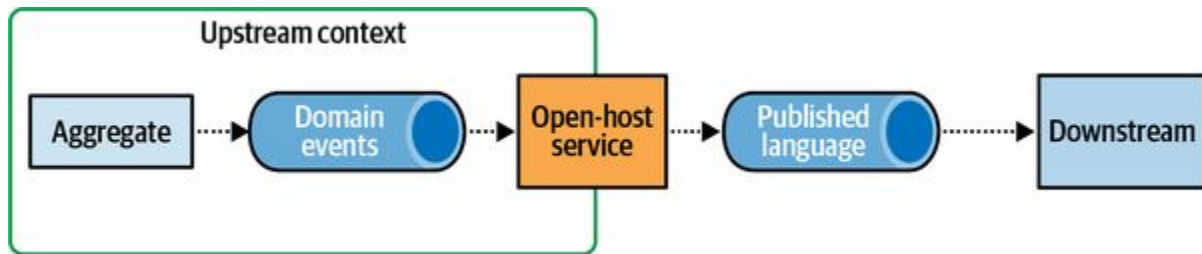
Figure 9-6. Domain events in a published language
