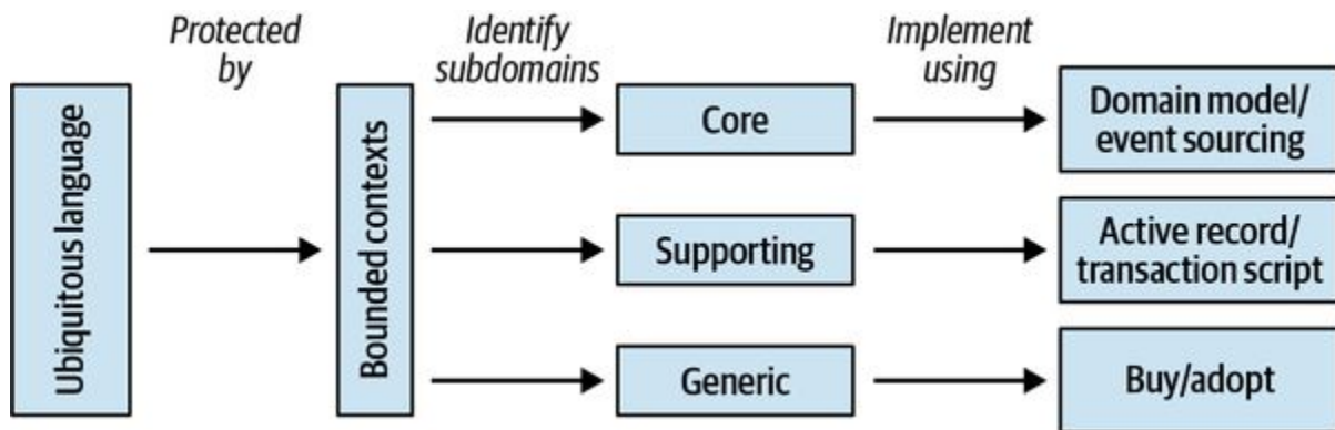
Figure A-6. A classic model of domain-driven design
