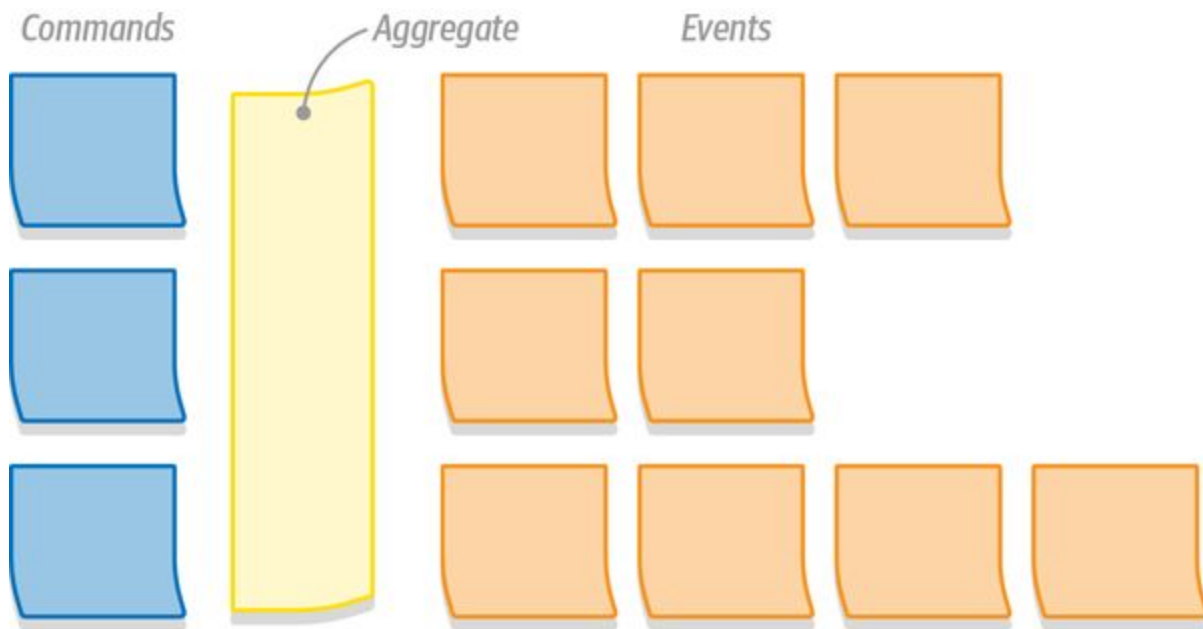
Figure 12-10. Commands and domain events organized in an aggregate
