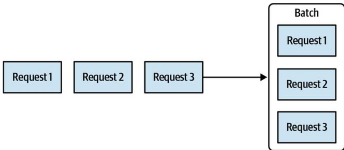
Figure 9-7. Batching requests
