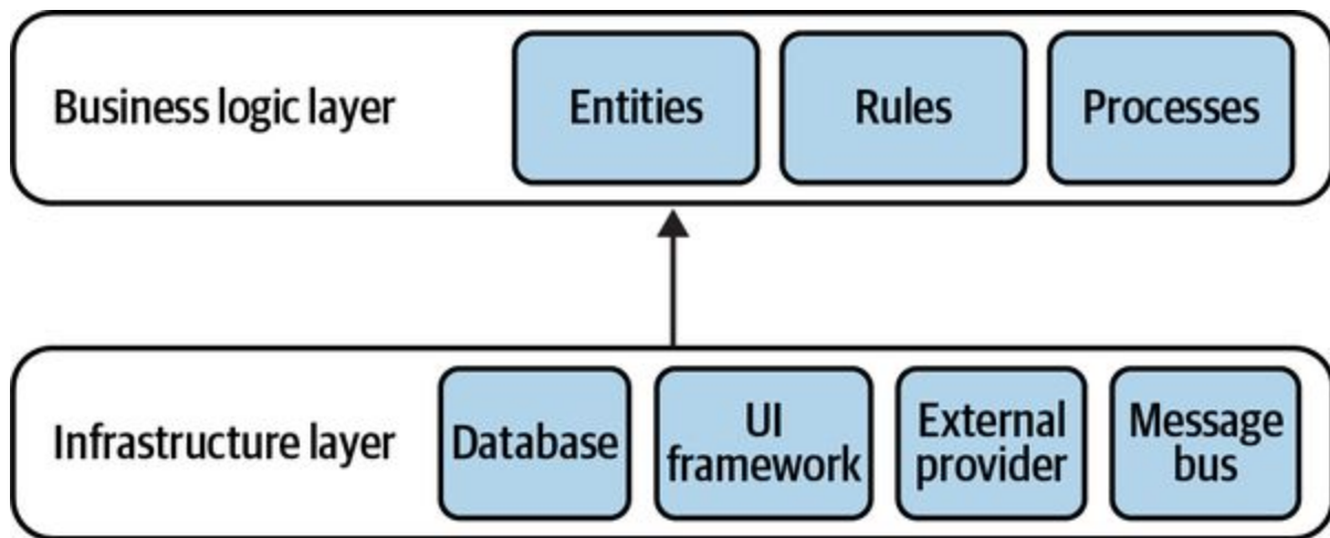
Figure 8-9. Reversed dependencies
