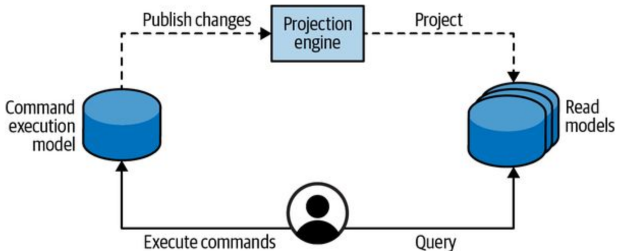
Figure 8-12. CQRS architecture
