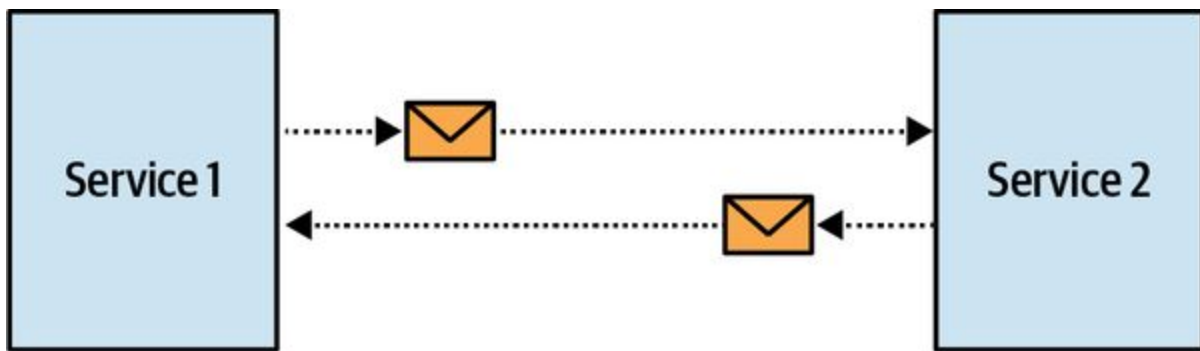
Figure 15-1. Asynchronous communication
