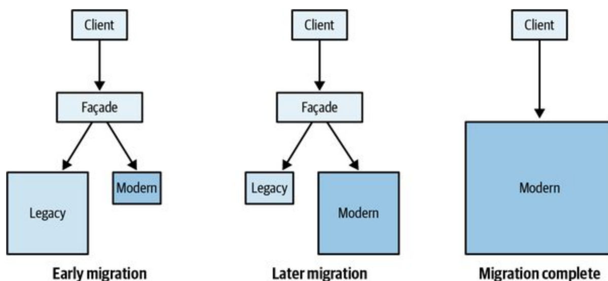
Figure 13-4. The façade layer forwarding the request based on the status of migrating the functionality from the legacy to the modernized system; once the migration is complete, both the façade and the legacy system are removed
