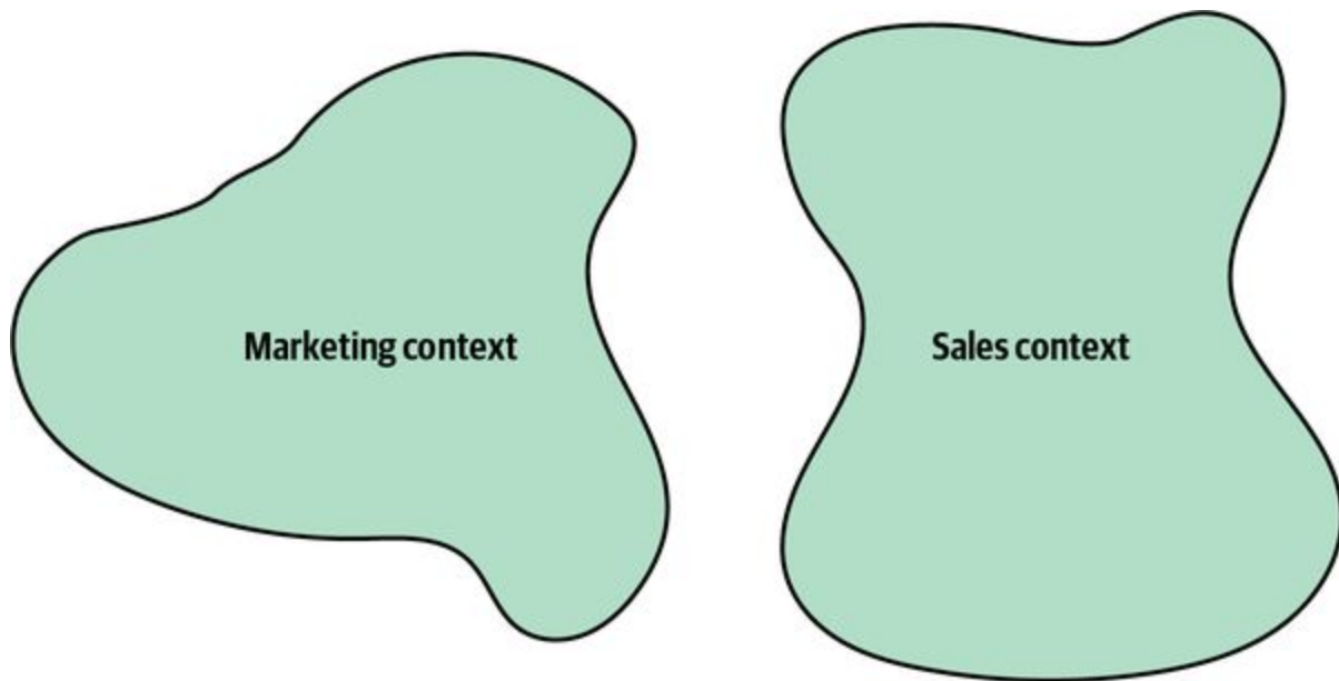
Figure 3-6. Bounded contexts driven by the consistency of the ubiquitous language
