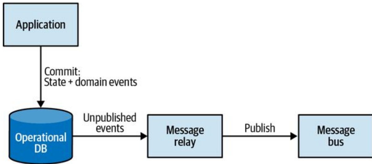
Figure 9-11. Outbox pattern
