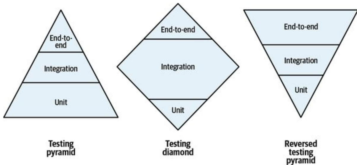
Figure 10-5. Testing strategies
