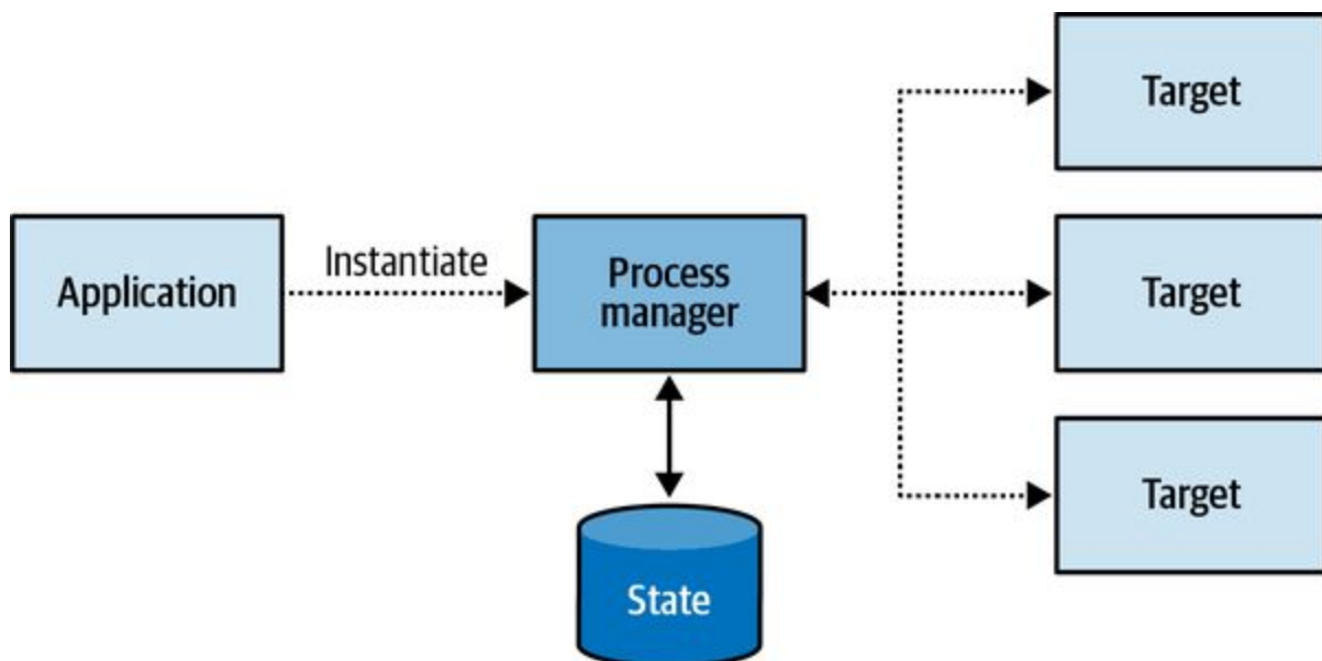
Figure 9-14. Process manager
