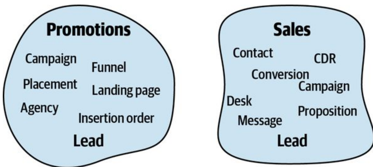
Figure 14-8. Bounded contexts
