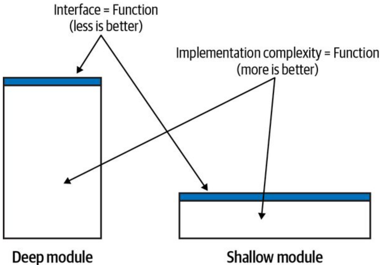
Figure 14-6. Deep modules
