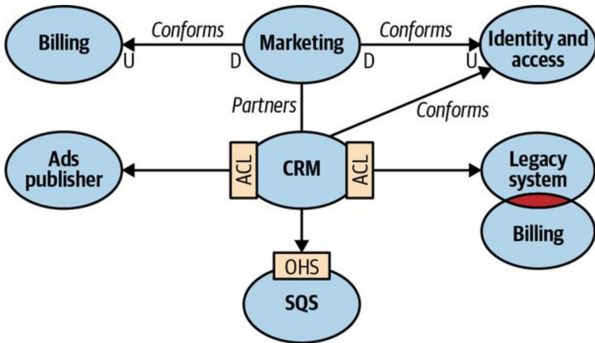
Figure 4-8. Context map
