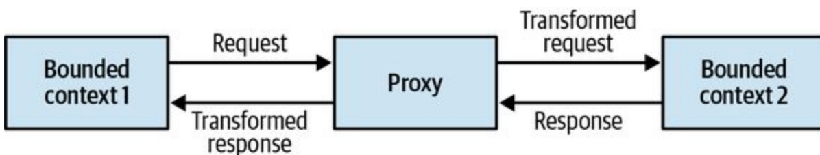
Figure 9-2. Synchronous communication
