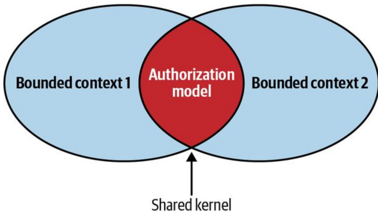
Figure 4-2. Shared kernel
