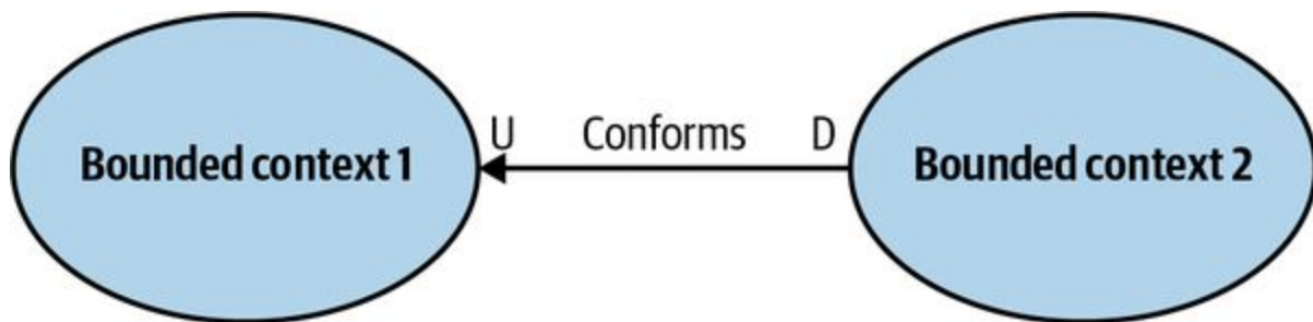
Figure 4-4. Conformist relationship
