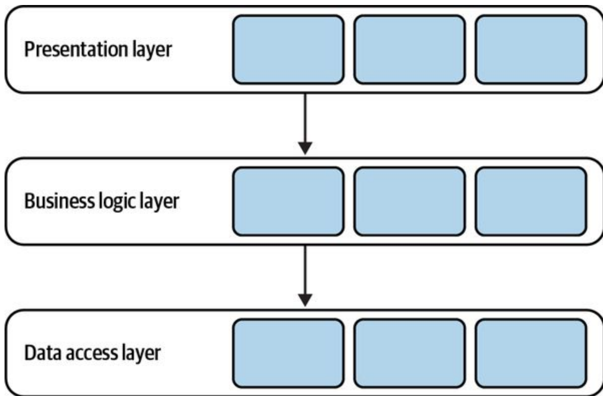
Figure 8-1. Layered architecture
