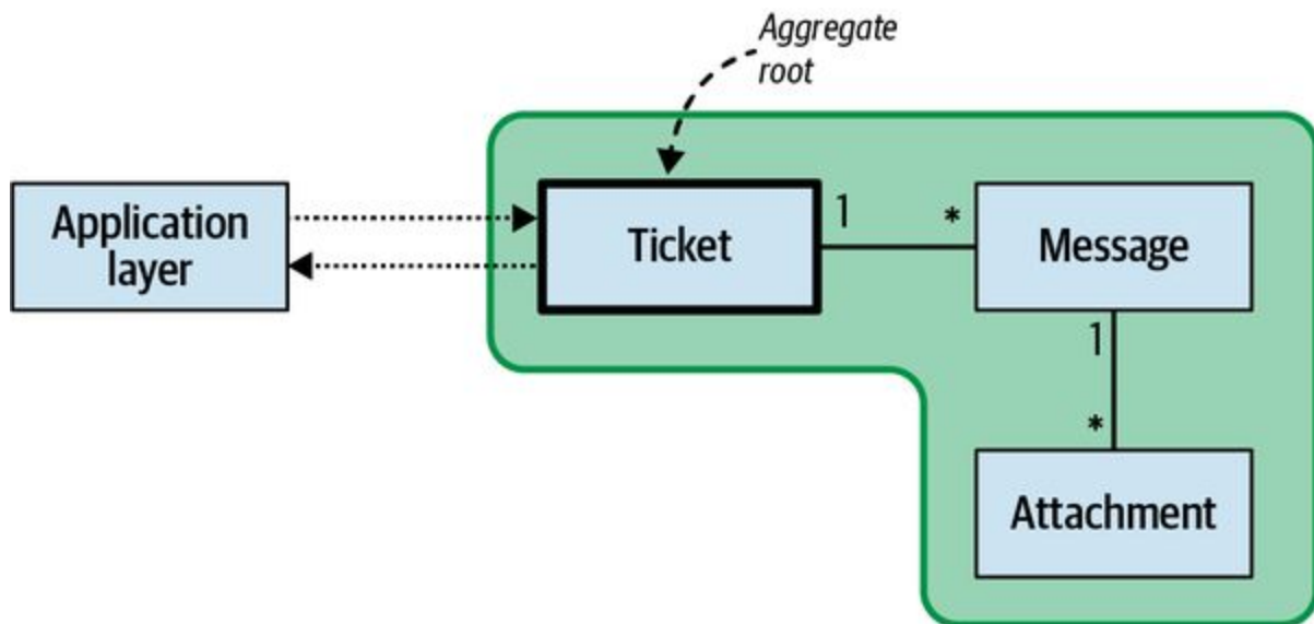
Figure 6-5. Aggregate root
