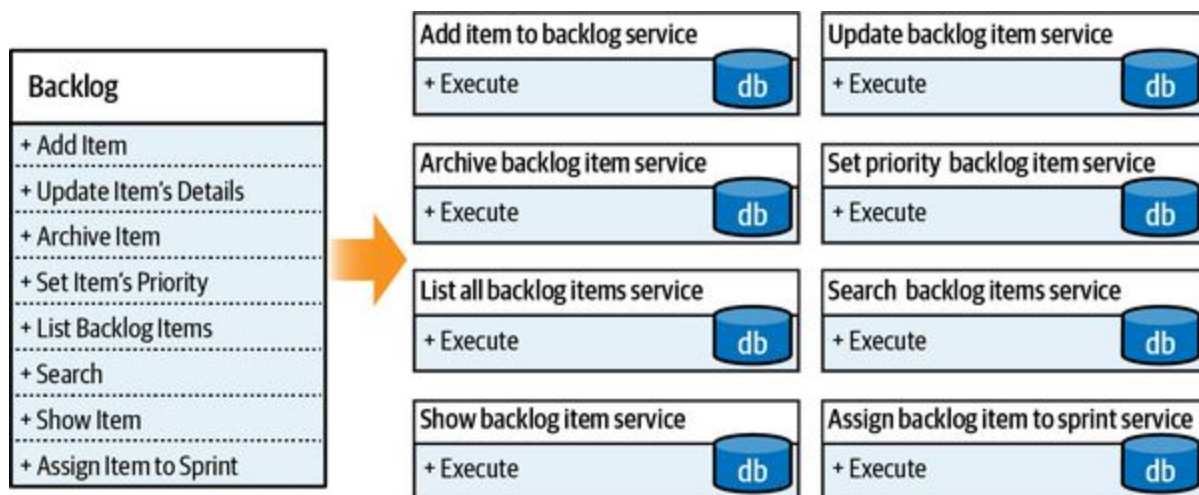
Figure 14-3. Naïve decomposition
