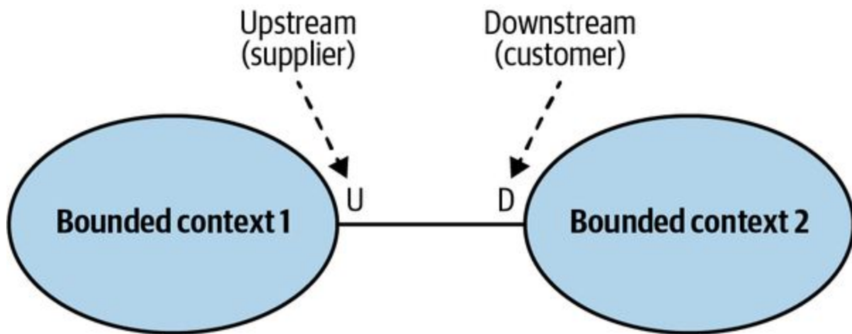
Figure 4-3. Customer–supplier relationship
