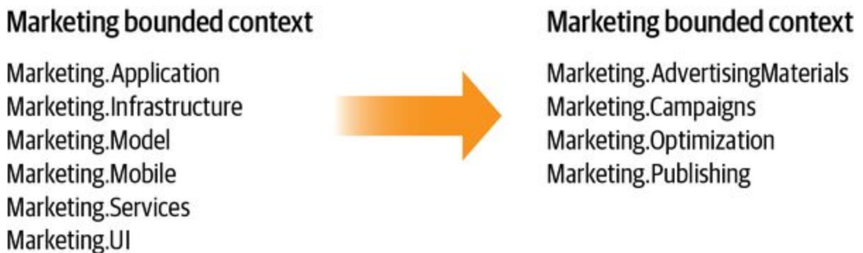
Figure 13-1. Reorganizing the bounded context’s modules to reflect the business subdomains’ boundaries rather than technical implementation patterns
