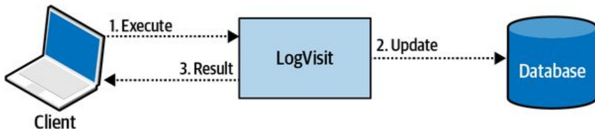
Figure 5-2. The LogVisit operation updating the data and notifying the caller of the operation's success or failure
