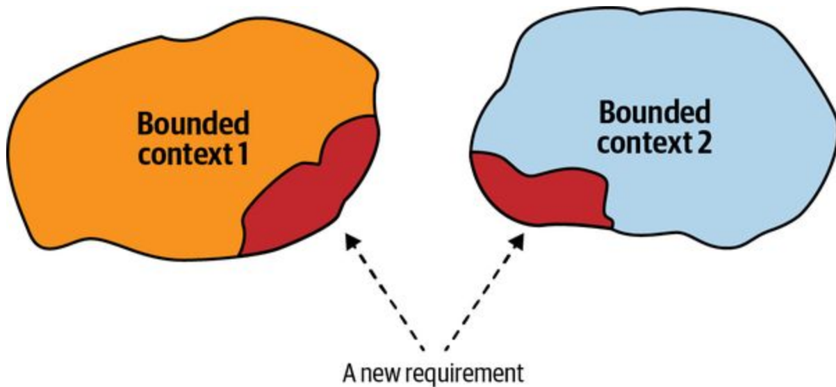
Figure 10-1. A change affecting multiple bounded contexts
