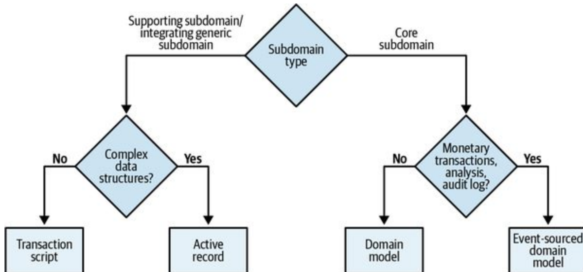
Figure 10-3. Decision tree for business logic implementation pattern
