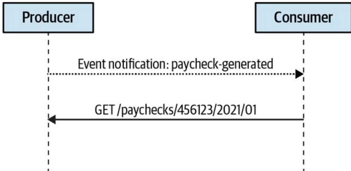
Figure 15-2. Event notification flow
