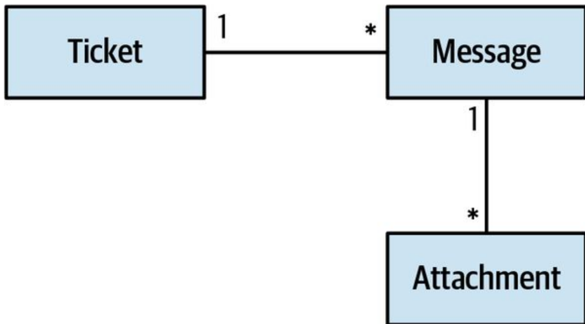
Figure 6-3. Aggregate as a hierarchy of entities
