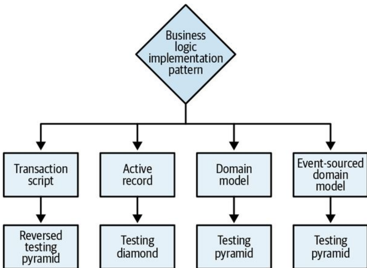
Figure 10-6. Testing strategy decision tree
