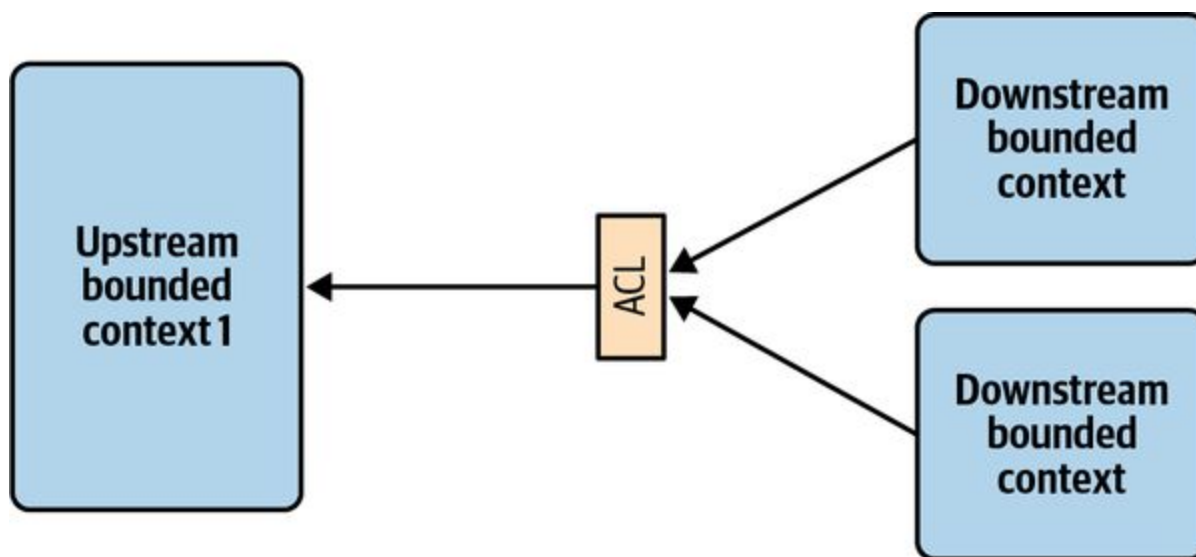
Figure 14-13. Anticorruption layer as a stand-alone service
