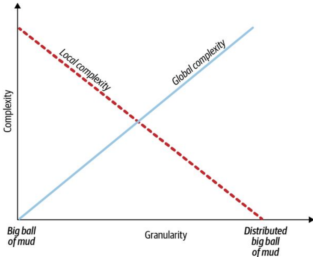
Figure 14-5. Service granularity and system complexities
