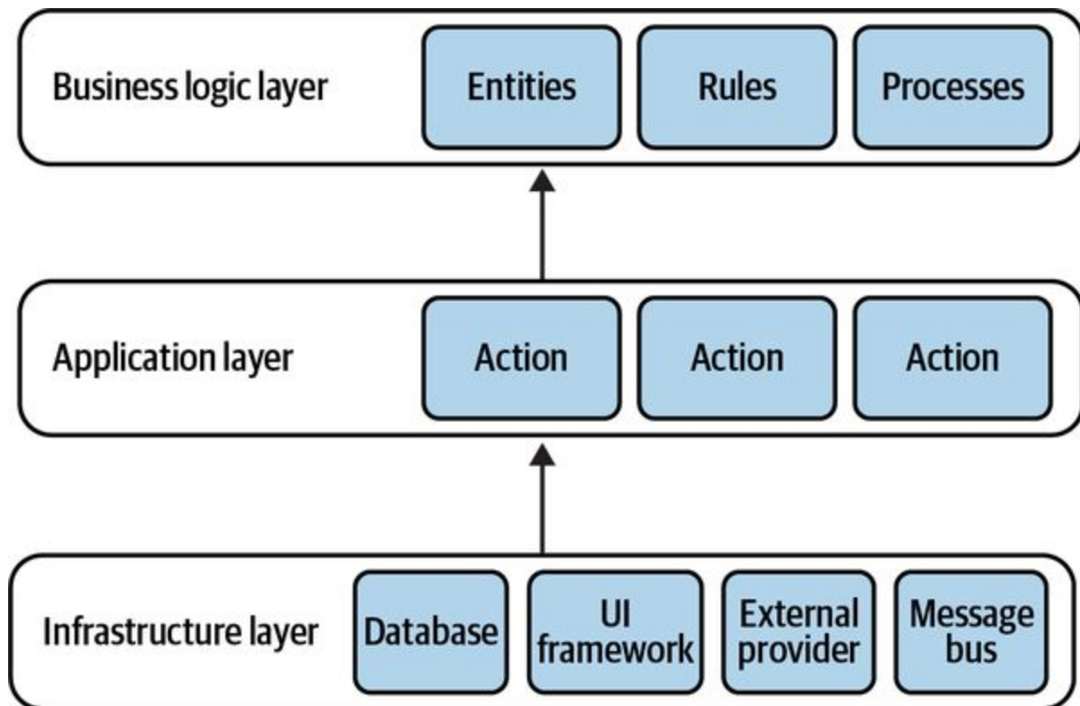
Figure 8-10. Traditional layers of the ports & adapters architecture
