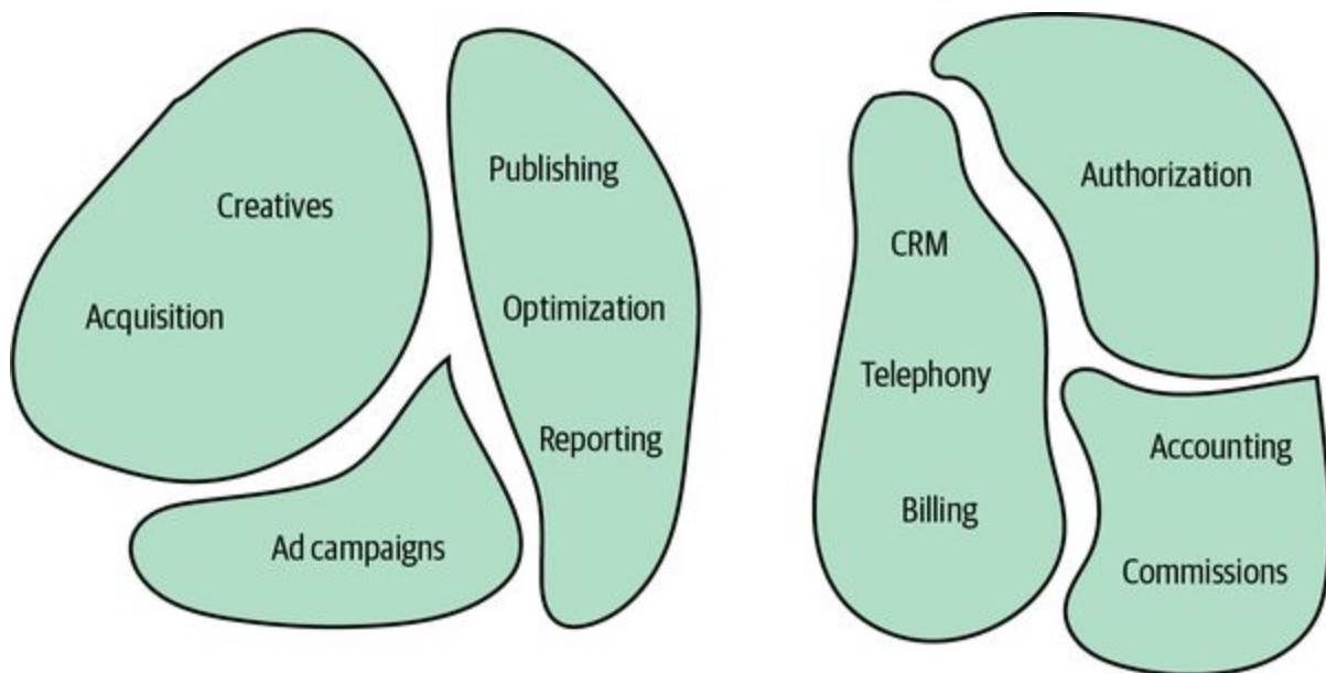
Figure 3-4. Smaller bounded contexts
