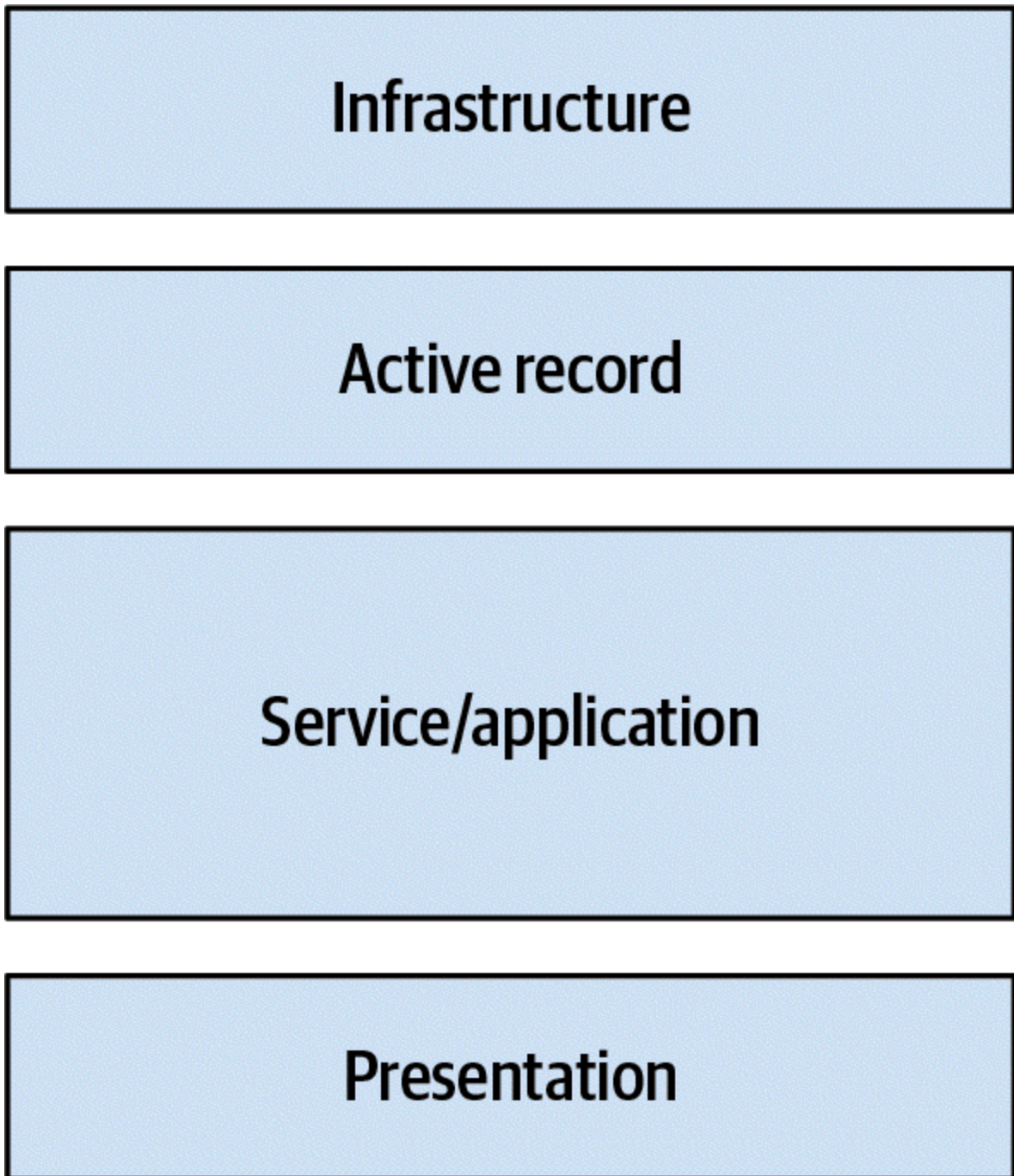
Figure A-5. The bonuses bounded context implemented using the active record and layered architecture patterns
