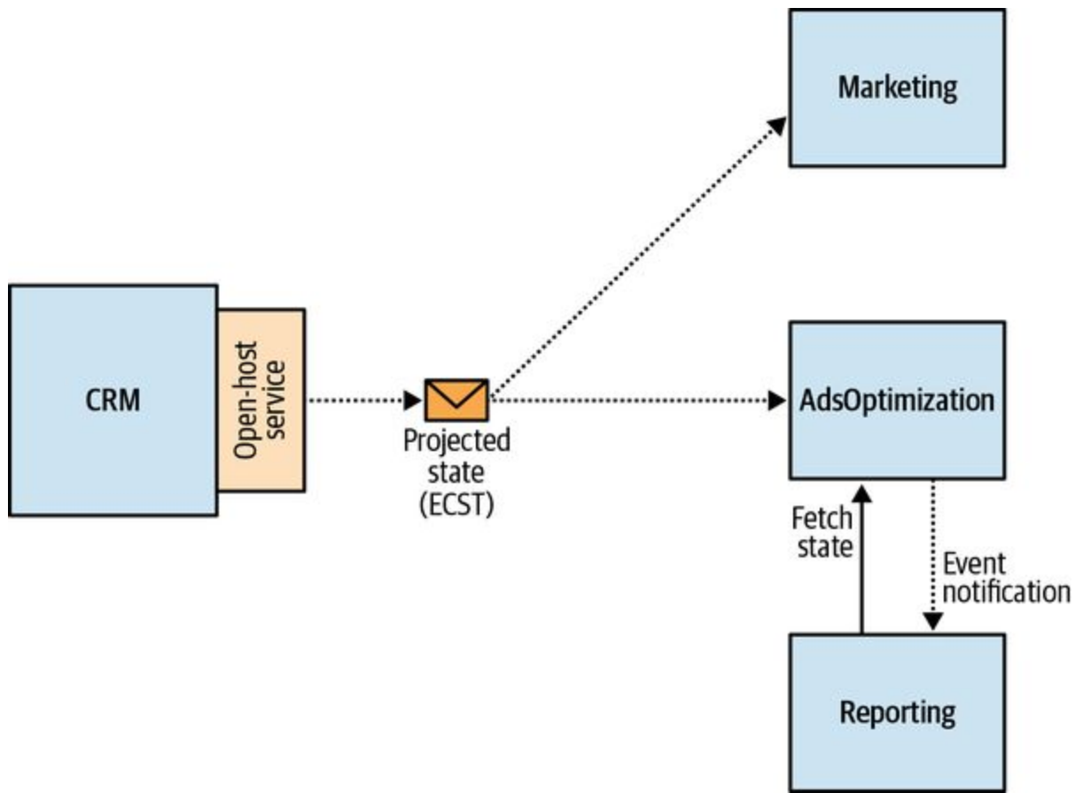
Figure 15-6. Refactored system
