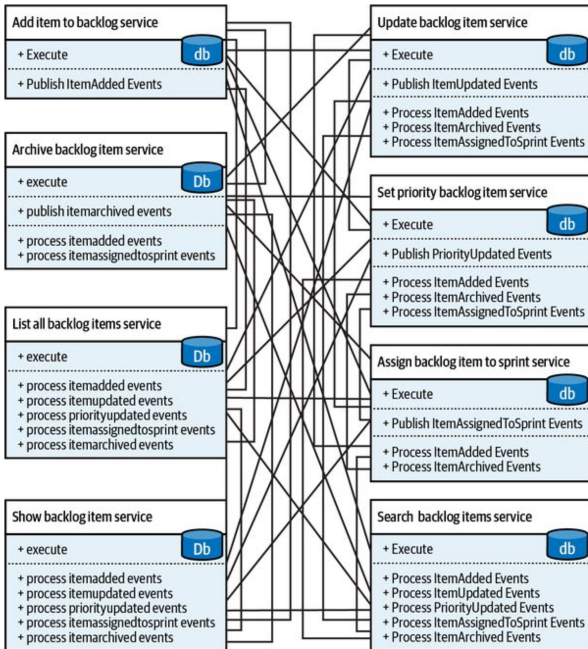
Figure 14-4. Integration complexity
