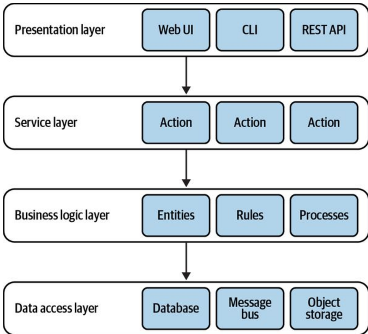
Figure 8-6. Service layer
