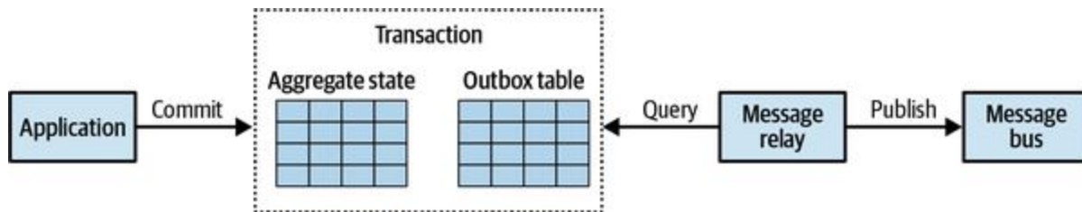
Figure 9-12. Outbox table
