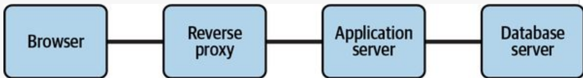
Figure 8-7. N-Tier system
