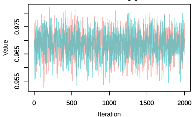
Trace – surv[3]
