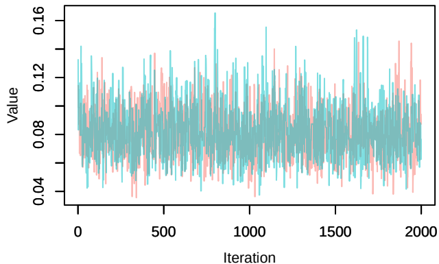
Trace – transi_31
