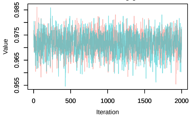
Trace – surv[2]
