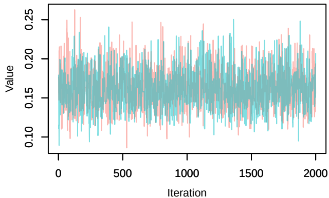
Trace – transi_13
