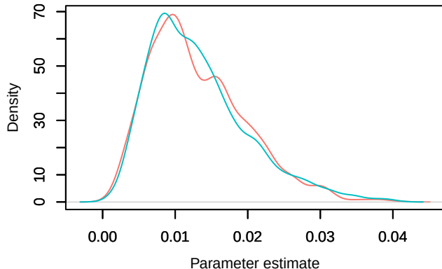
Density – transi_32
