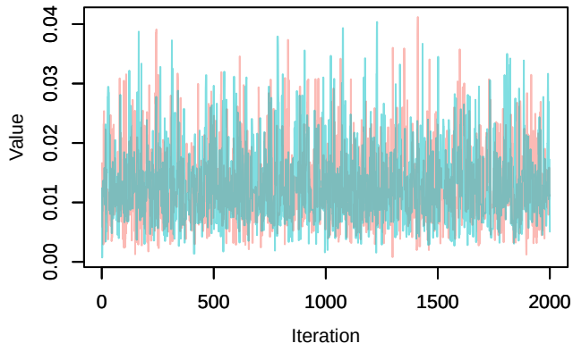
Trace – transi_32
