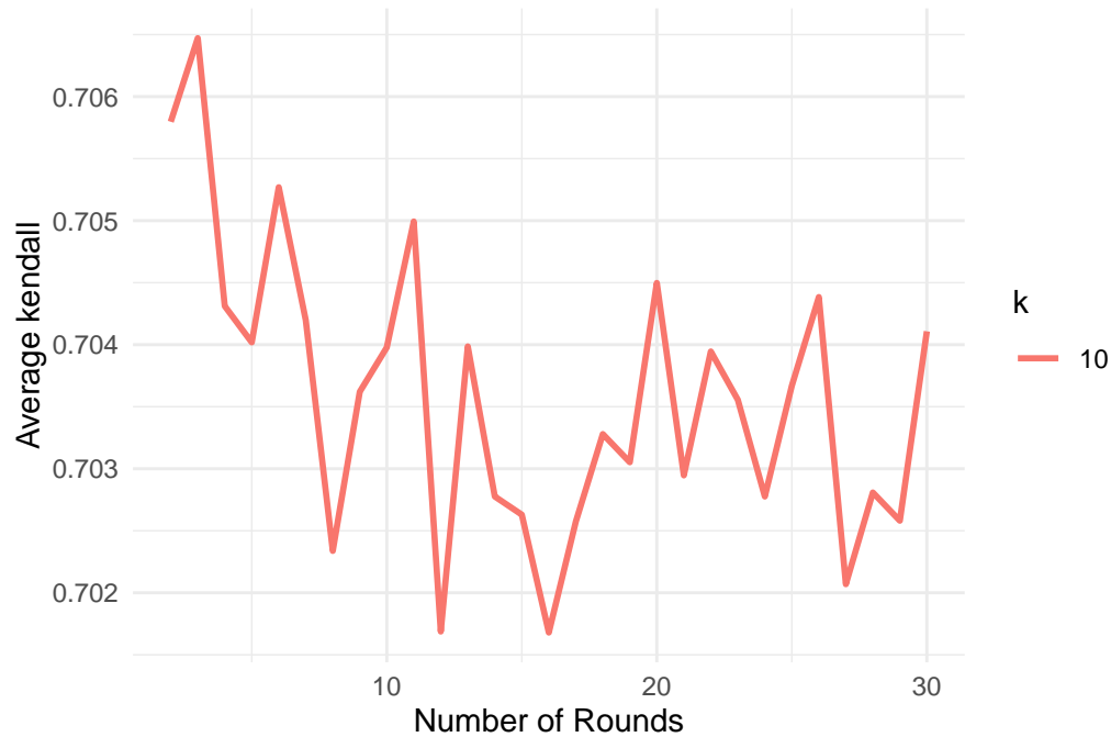
Average kendall vs Number of Rounds
