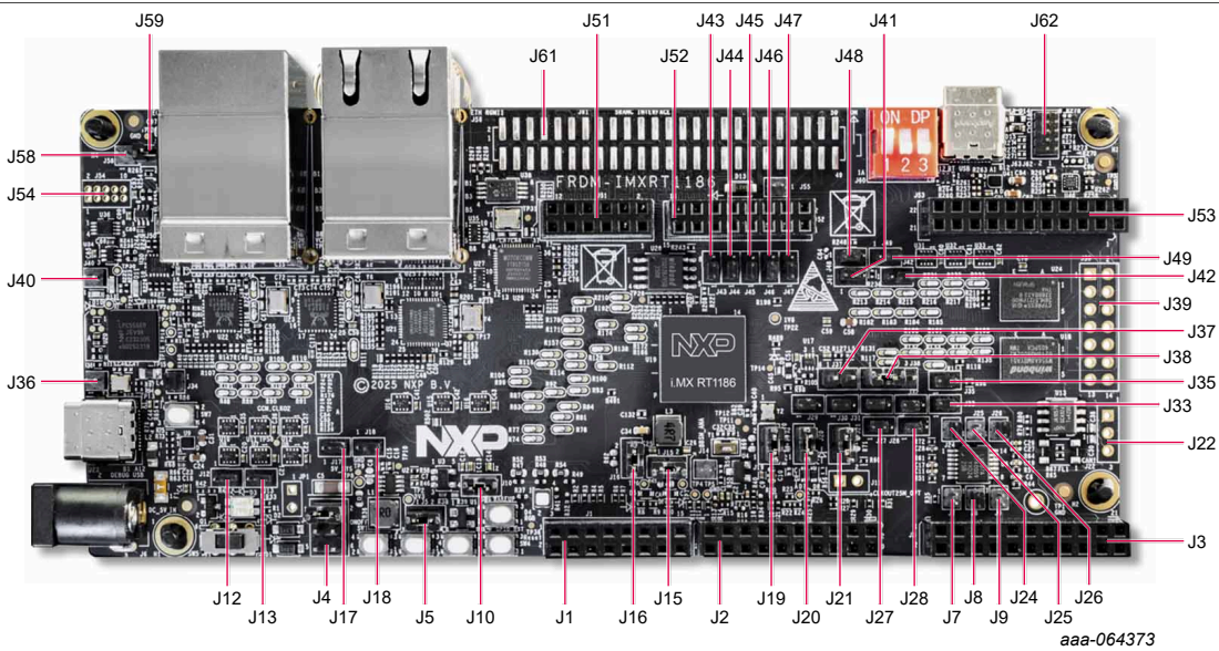
Figure 4. FRDM-IMXRT1186 board connectors and jumpers
