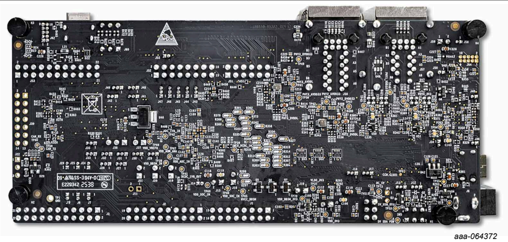
Figure 3. Bottom view of the FRDM-IMXRT1186 board
