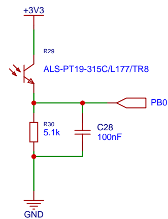
LIGHT SENSOR
