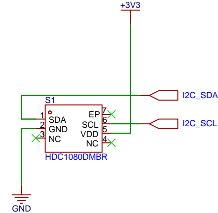
TEMP & HUMIDITY
