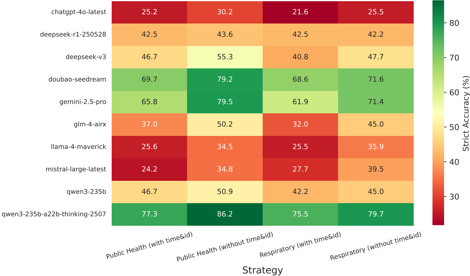
Model Performance Heatmap
