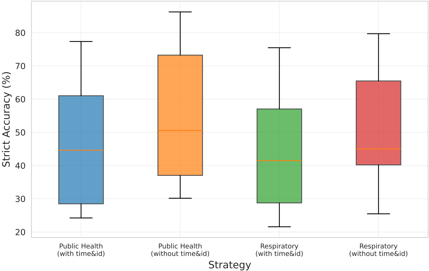
Strategy Performance Distribution
