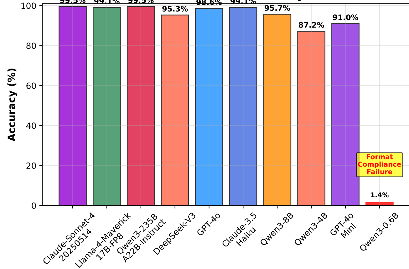
Direct Answer Accuracy
