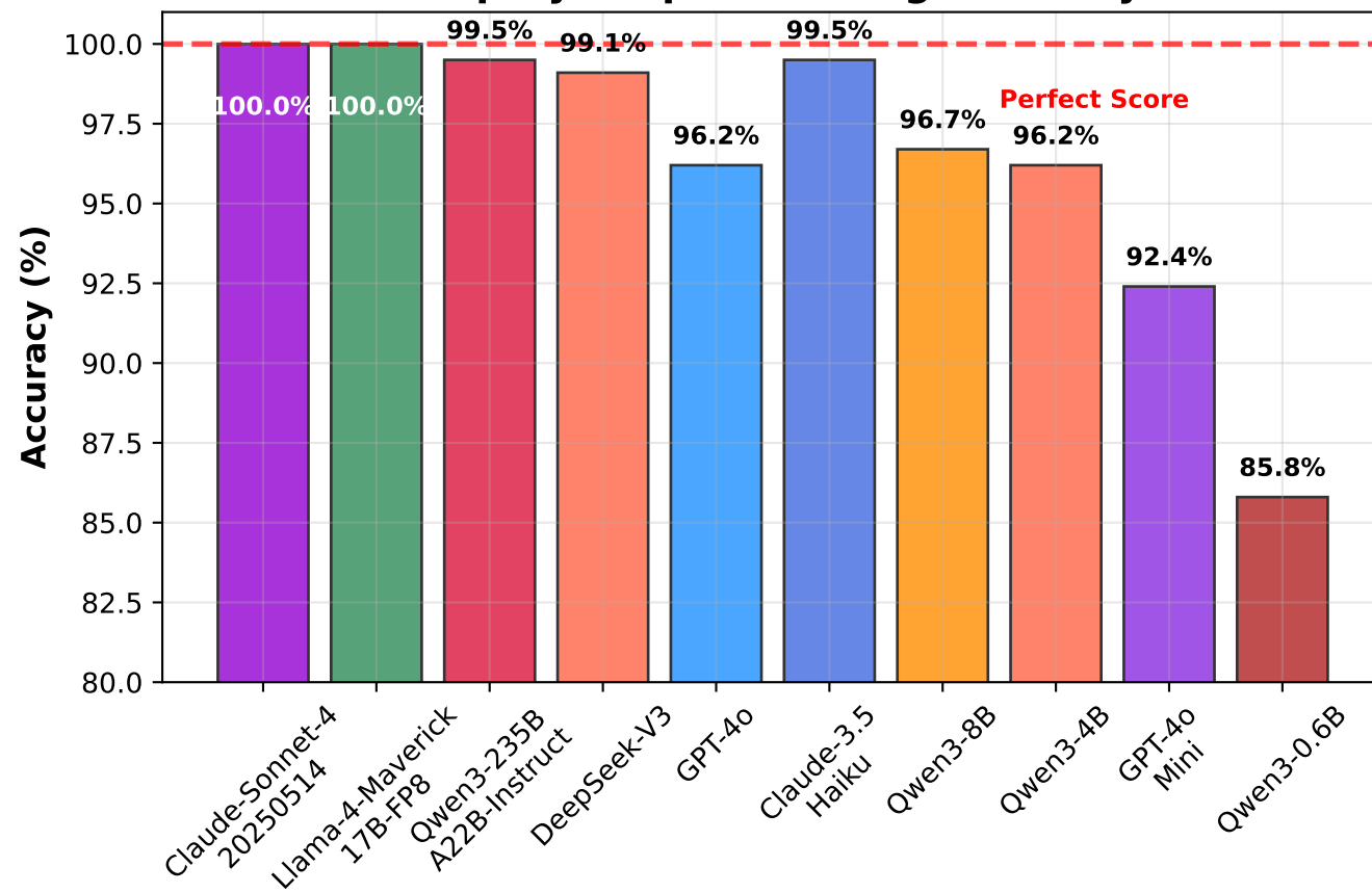
Step-by-Step Reasoning Accuracy
