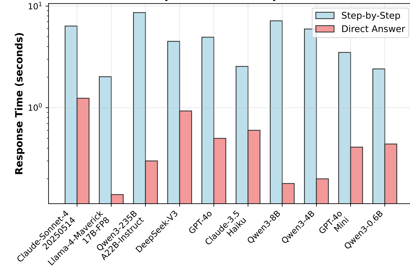
Response Time Comparison
