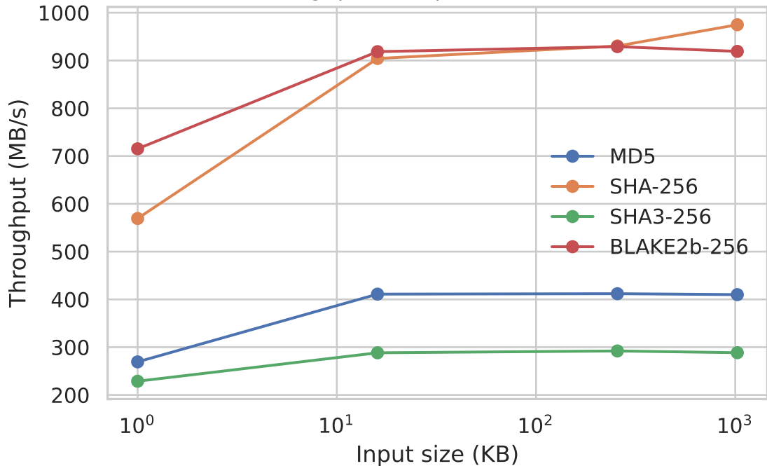
Hash Throughput vs Input Size (random data)
