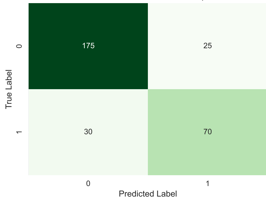
Fairness-Aware Model - Group 0
