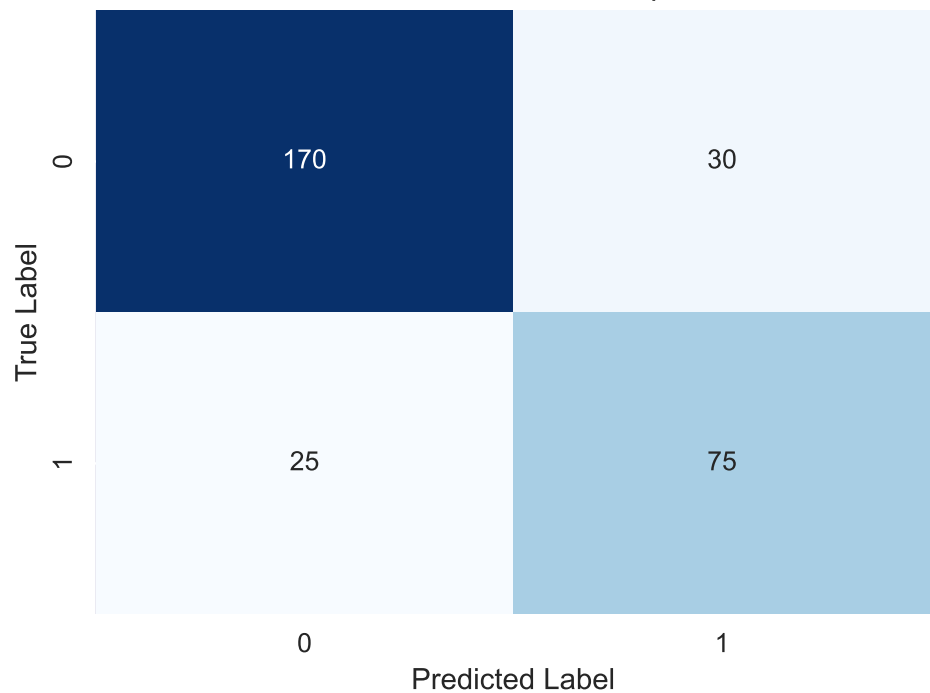
Fairness-Aware Model - Group 1
