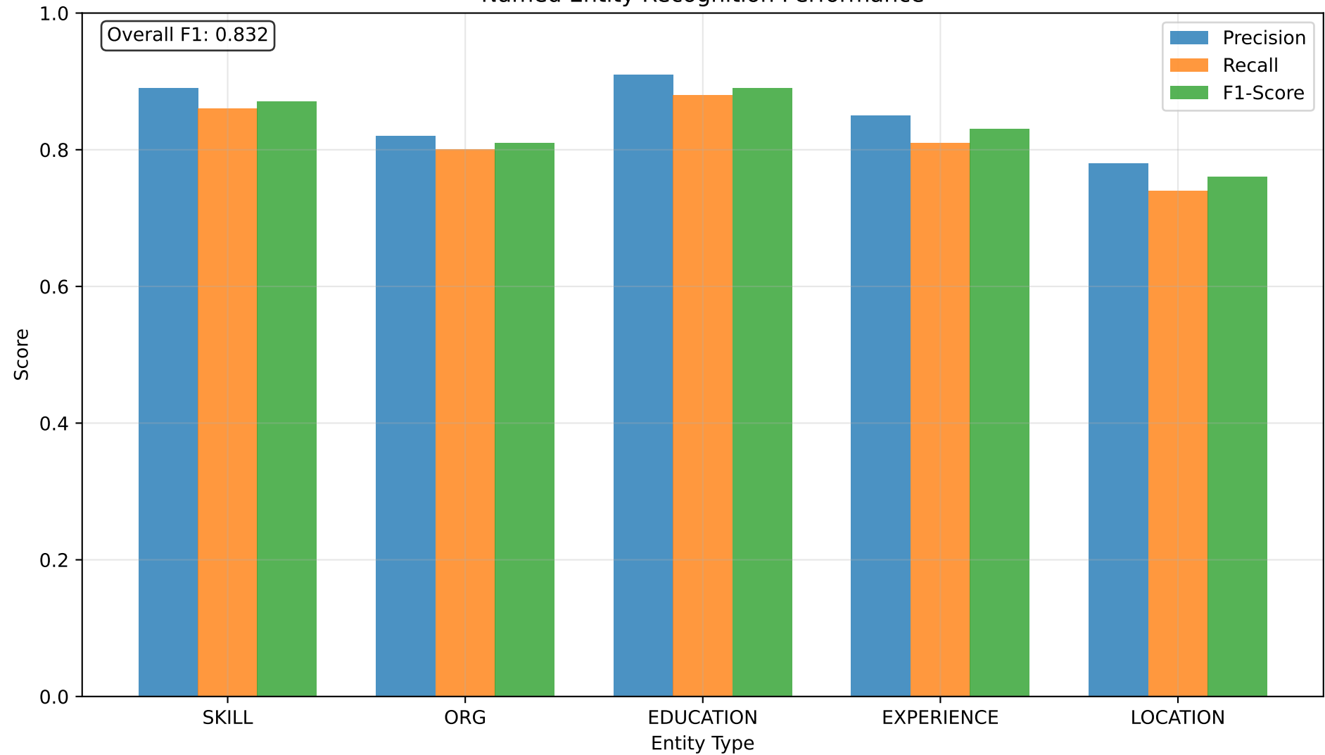
Named Entity Recognition Performance
