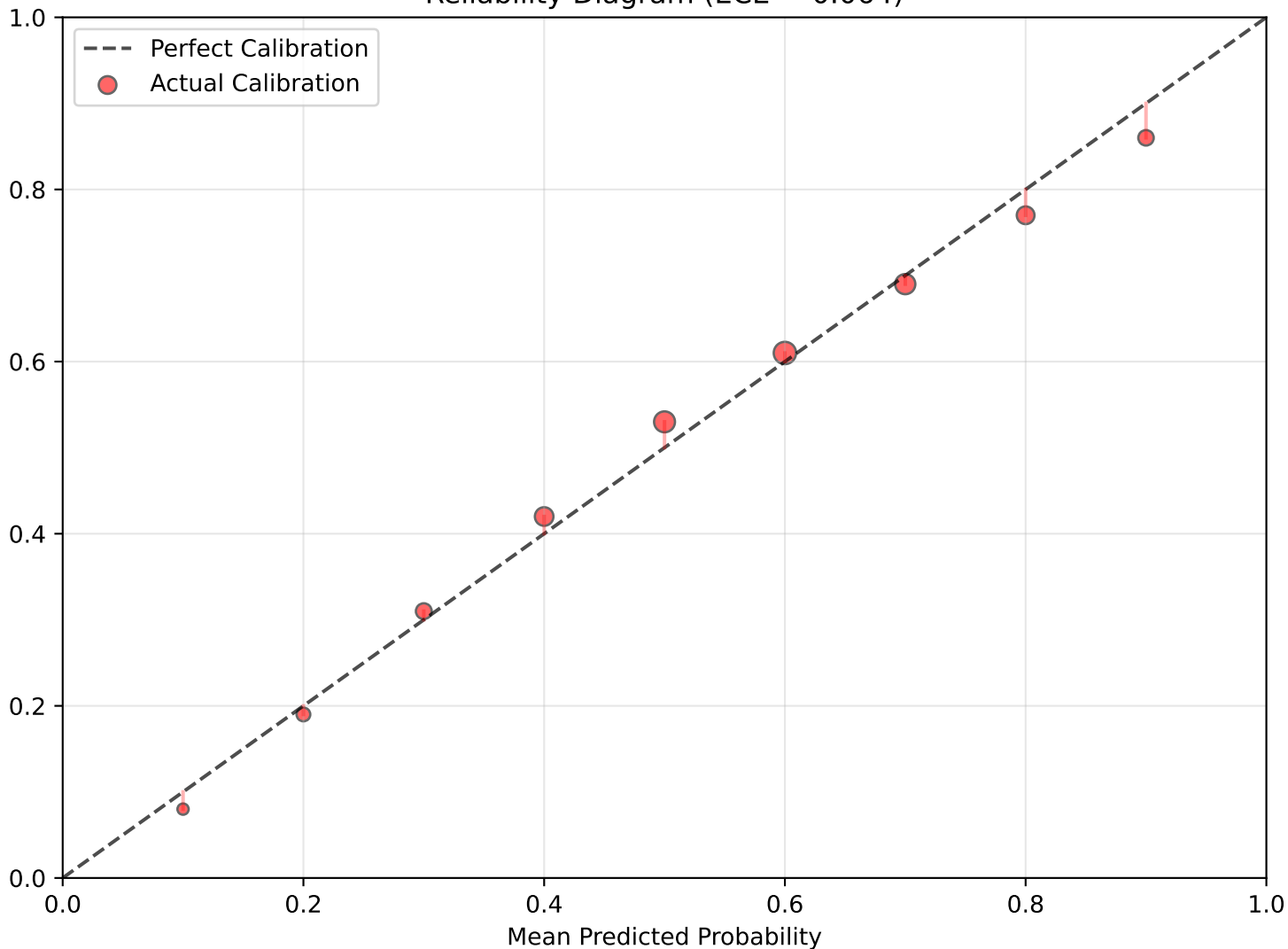
Reliability Diagram (ECE = 0.064)
