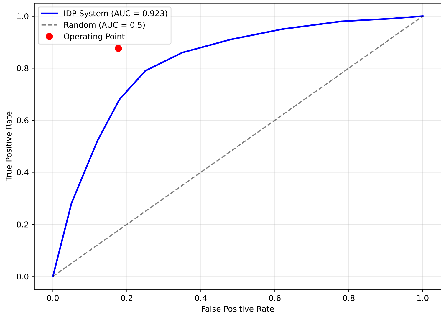
ROC Curve - Academic Decision Classification
