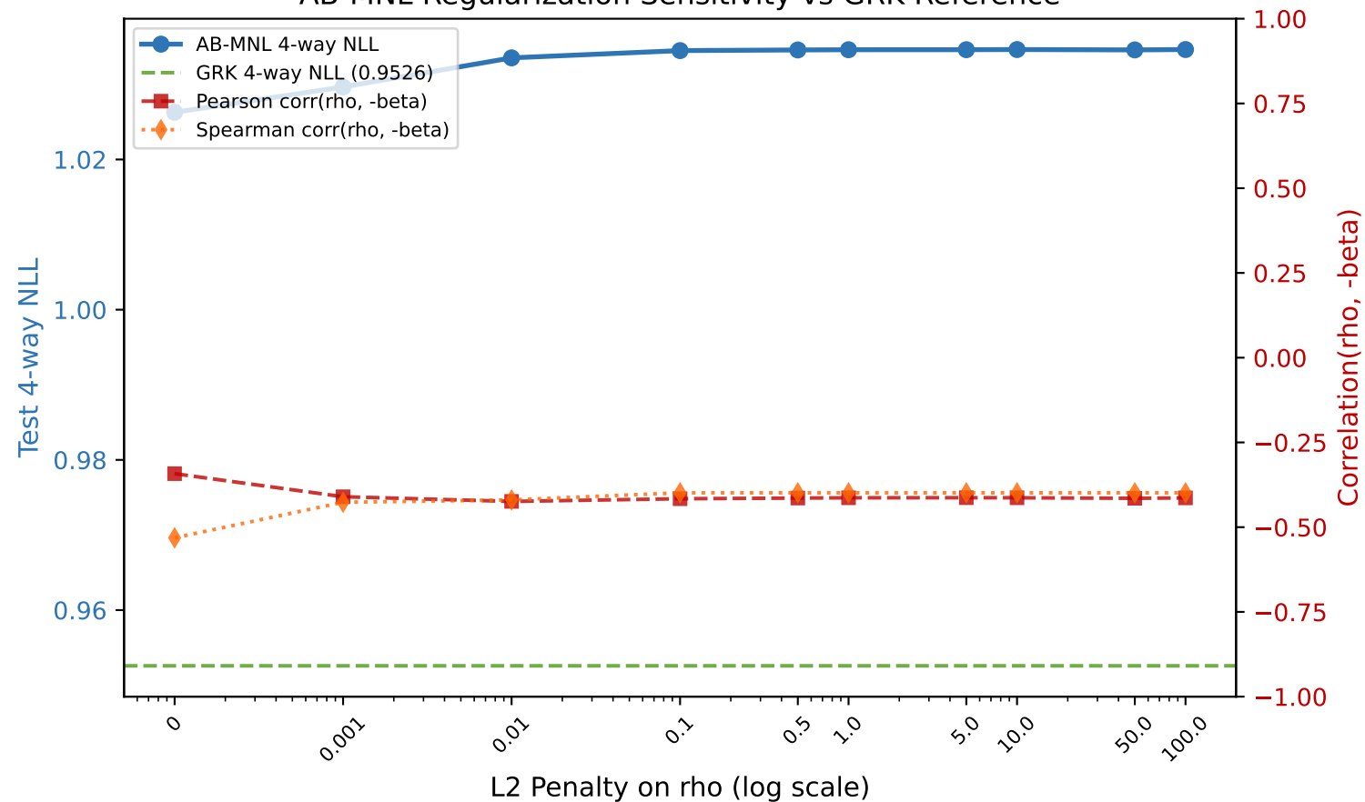
AB-MNL Regularization Sensitivity vs GRK Reference
