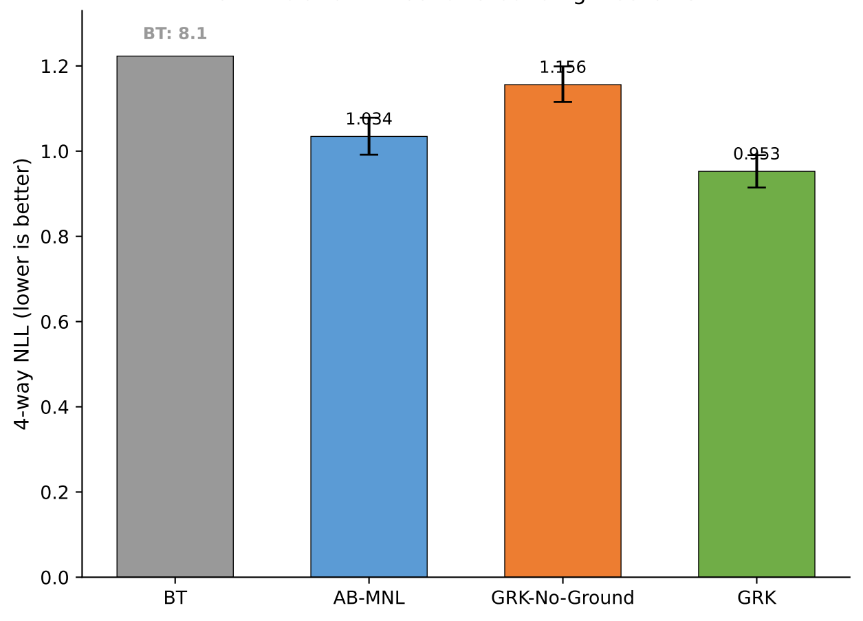
GRK Ablation: Effect of Grounding Mechanism
