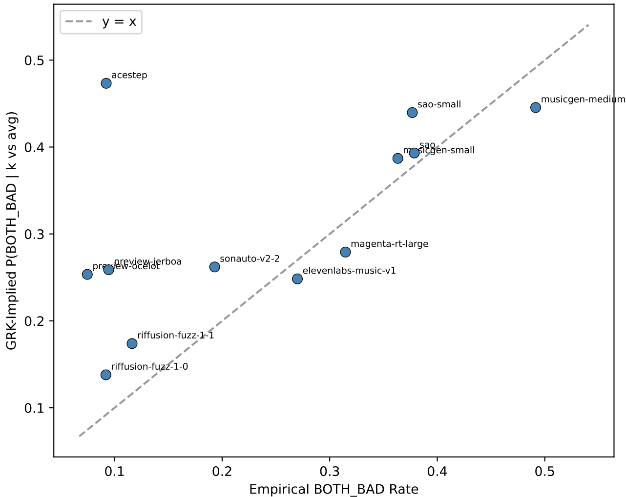
GRK Acceptability vs Empirical Pearson r=0.597 , Spearman r=0.566
