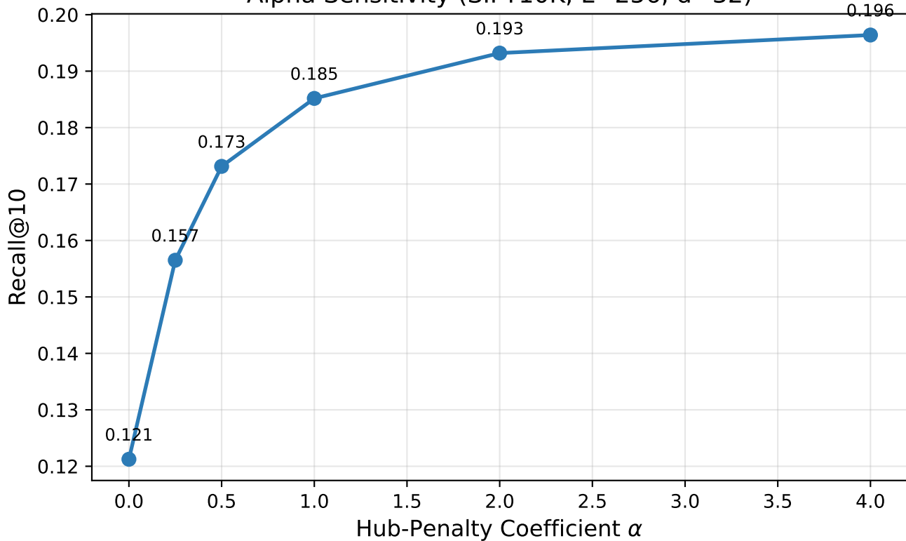
Alpha Sensitivity (SIFT10K, L=256, d=32)
