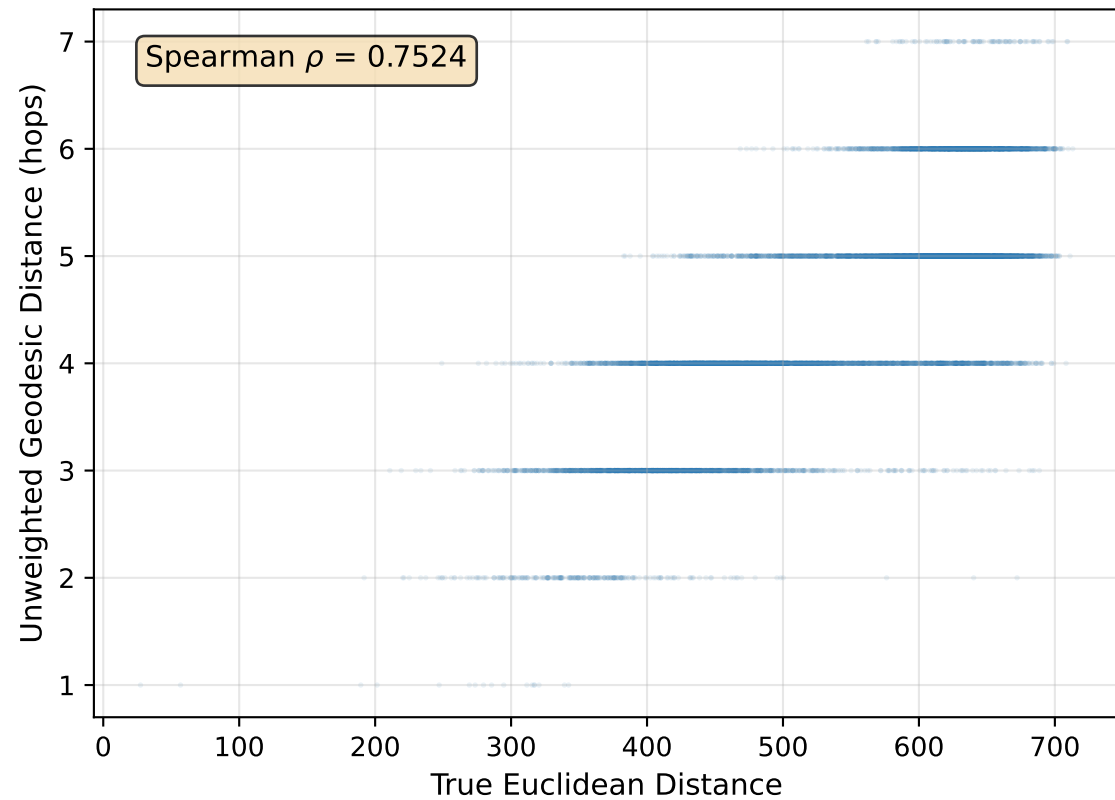
Unweighted Geodesic vs Euclidean
