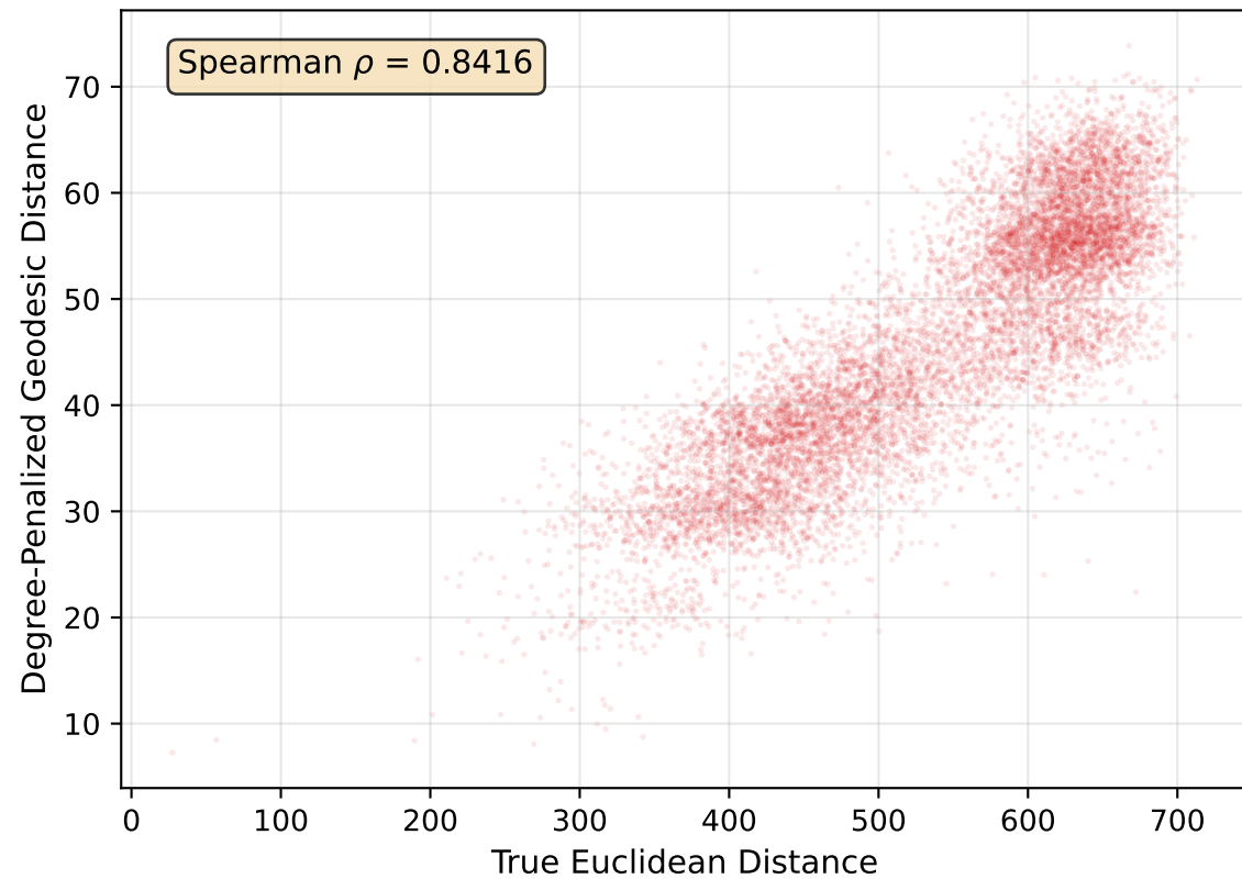
Degree-Penalized Geodesic ( \alpha=3.0 ) vs Euclidean
