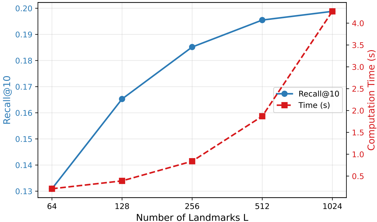
Landmark Sensitivity (SIFT10K, \alpha=1.0 , d=32 )
