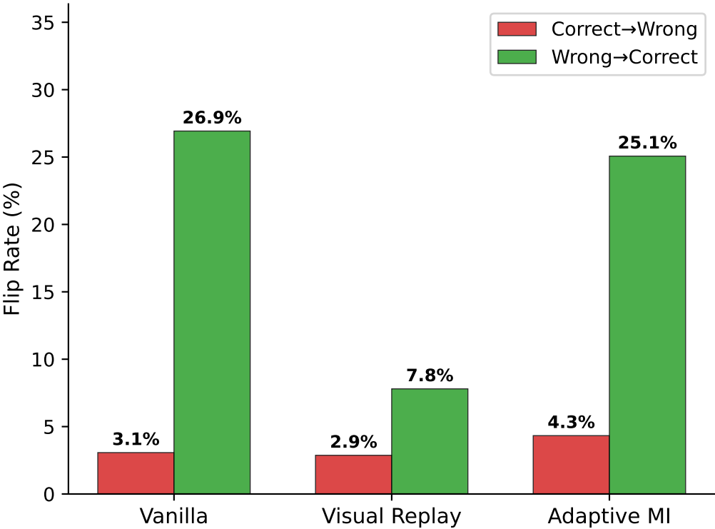
Flip Rates on MMSTAR (128→512 tokens)
