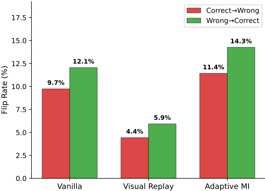
Flip Rates on HALLUSIONBENCH (128→512 tokens)
